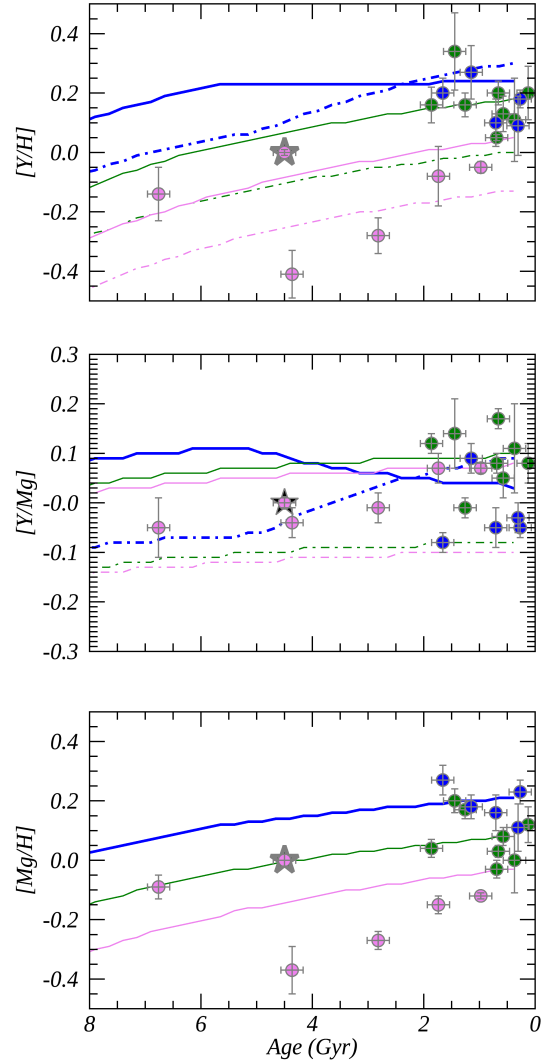
Fig. 2. [Y/H] , [Y/Mg] , and [Mg/H] vs. age: sample of Gaia -ESO IDR5 clusters in three radial bins ( R_{GC} < 6.5 kpc in blue, 6.5 \text{ kpc} < R_{GC} < 9 kpc in green, and R_{GC} > 9 kpc in pink) compared with results of the GCE for the thin disc at three R_{GC} = 6, 8 , and 10 kpc with the MAGN yields (continuous curves) and with the FRUITY yields (dot-dashed lines). The ages and R_{GC} of open clusters are from Cantat-Gaudin et al. (2020). The star marks the abundance ratio at the solar age and Galactocentric distance.
