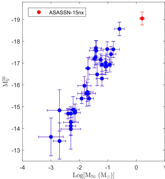
Figure 11. Absolute V-band magnitude at t = 50 days as a function of the estimated ^{56}\text{Ni} mass for the SNe II sample, from Hamuy (2003) and Spiro et al. (2014). ASASSN-15nx, shown with a red dot, lies on the extrapolation of the correlation to higher masses and luminosities.
