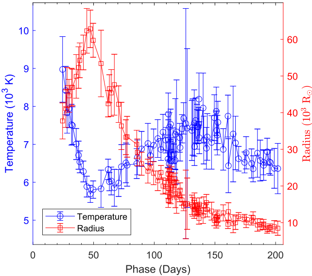
Figure 8. Temporal evolution of the blackbody temperature (blue, left scale) and radius (red, right scale) of ASASSN-15nx.
