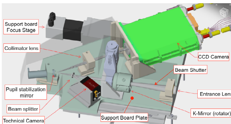
Figure 5. NGS WFS unit. The unit cover is hidden to show the content.
