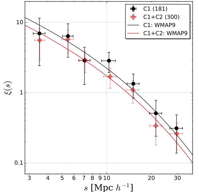
Fig. A.2. Comparison between the redshift-space 2PCF of XXL C1 (black dots) and C1+C2 clusters (red diamonds). The black and red lines show the theoretical WMAP9 predictions, computed as described in Sect. 4 for C1 and C1+C2, respectively. The number of C1 and C1+C2 XXL clusters in each field is reported in parentheses.
