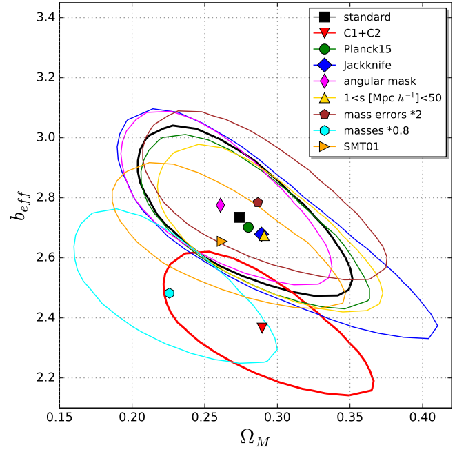
Fig. A.5. 1\sigma MCMC confidence contours of \Omega_M - b_{\text{eff}} obtained with different assumptions: standard analysis, as described in Sect. 4 – black; considering C1+C2 XXL clusters, instead of C1 only – red; assuming Planck15 as reference cosmology, instead of WMAP9 – green; with jackknife covariance, instead of bootstrap – blue; considering the angular mask to construct the random catalogue, instead of the technique described in Sect. 3.3 – magenta; considering the fitting scale range 1 < r[h^{-1} \text{ Mpc}] < 50 , instead of 10 < r[h^{-1} \text{ Mpc}] < 40 – yellow; doubling the statistical mass errors – brown; reducing the masses by 20% – cyan; assuming the Sheth et al. (2001) bias model to compute the effective bias of the sample – orange.
