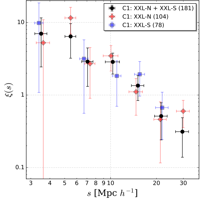
Fig. A.1. Comparison between the redshift-space 2PCF of XXL C1 in XXL-N (red diamonds), in XXL-S (blue squares), and in the whole sample (black dots). The number of XXL clusters in each field is reported in parentheses. The error bars are as in Fig. 3.
