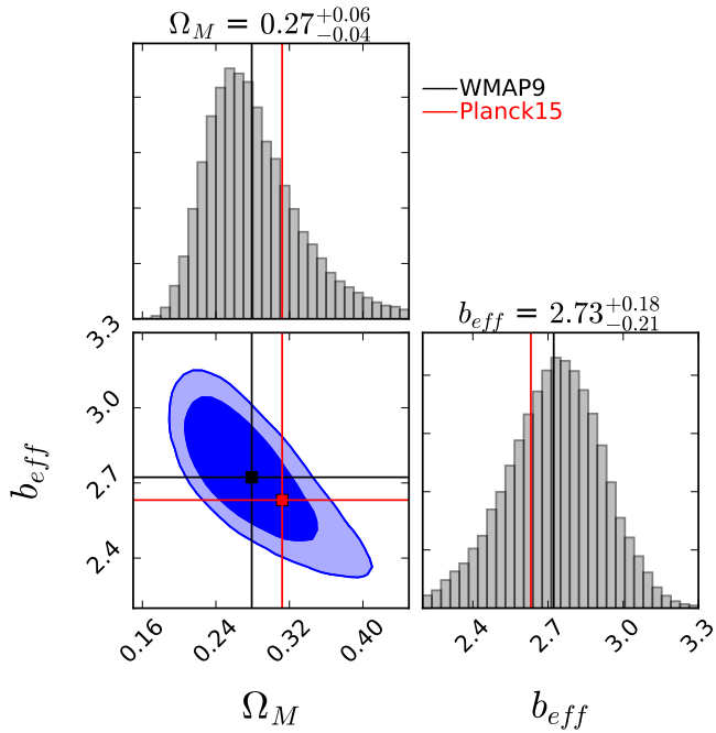
Fig. 5. Confidence contours ( 1 - 2\sigma ) of \Omega_M - b_{\text{eff}} provided by the MCMC, as described in Sect. 4 ( b_{\text{eff}} is a derived parameter, the ellipse width corresponds to the deviation of the \sigma_8 Gaussian prior). The histograms (top and bottom right panels) show the posterior distributions of \Omega_M and b_{\text{eff}} , respectively. Black and red lines represent WMAP9 and Planck15 predictions, respectively.
