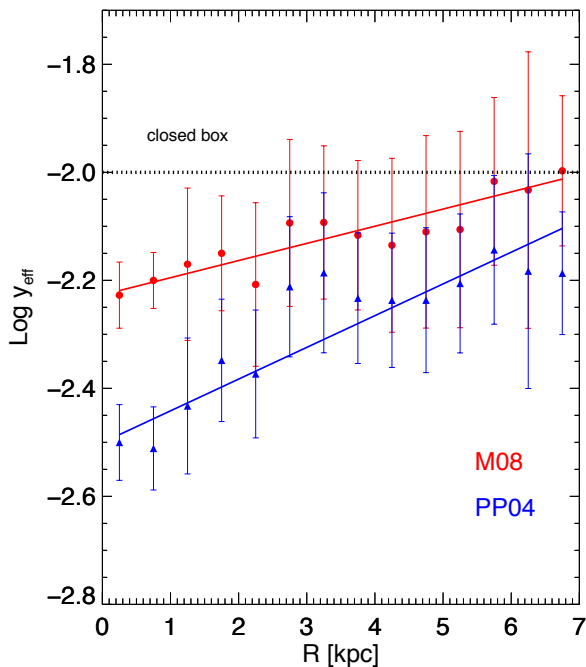
Figure 4. The radial variation of the effective yield in NGC 628. The value expected for the closed box case, y/(1 - R) = 0.010 , is indicated as a black dotted line. The red circles and blue triangles represent respectively the results obtained with the Maiolino et al. (2008) and Pettini & Pagel (2004) calibrations.
