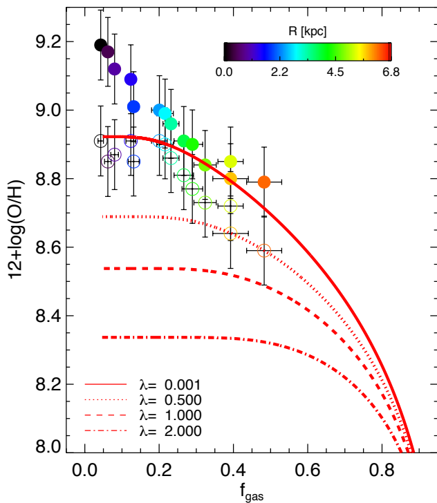
Figure 7. Gaseous metallicity 12 + \log(\text{O}/\text{H}) versus gas fraction. Symbols show the values observed in radial annuli in NGC 628, where the colour-coding gives the galactocentric radial distance, as indicated in the colour bar. Solid symbols correspond to the mass of metals in which the ISM metallicity is calculated by using the M08 calibration, while open symbols use the PP04 calibration. The red lines correspond to the prediction of simple chemical evolution models with different values for the average outflow loading factor ( \lambda ). Note that the model relations are independent of the inflow rate \Phi and of the star formation efficiency \epsilon .
