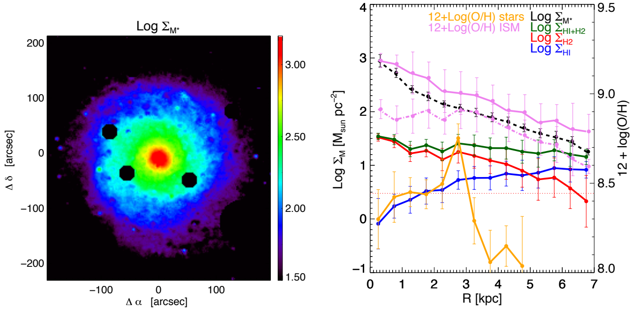
Figure 3. Left: Stellar mass surface density map, created from the spatially resolved SED fitting. Foreground stars have been masked. Right: Radial dependance of various physical quantities across the disk of NGC 628 (in radial bins; error bars represent the scatter in each radial bin). Atomic gas surface density (blue) shows a dip in the central region, while the molecular gas surface density (red) is peaked at the centre and quickly decreases outwards. The horizontal red dashed line corresponds to the sensitivity limit of the CO observations. The total gas content (green) is nearly flat across the whole disk up to 3 R_e ( 1 R_e = 2.4 \text{ kpc} ). A clear radial gradient is observed in both stellar mass surface density (black, short dashes) and gas metallicity (violet). The latter is shown both for the M08 (solid violet) and PP04 (dot-dashed violet) metallicity calibrations. The stellar metallicity gradient from Sanchez-Blazquez et al. (2014) is shown in orange. Note that the metallicities of gas and stars are plotted with respect to the alternative y-axis on the right in units of 12 + \log(\text{O}/\text{H}) .
