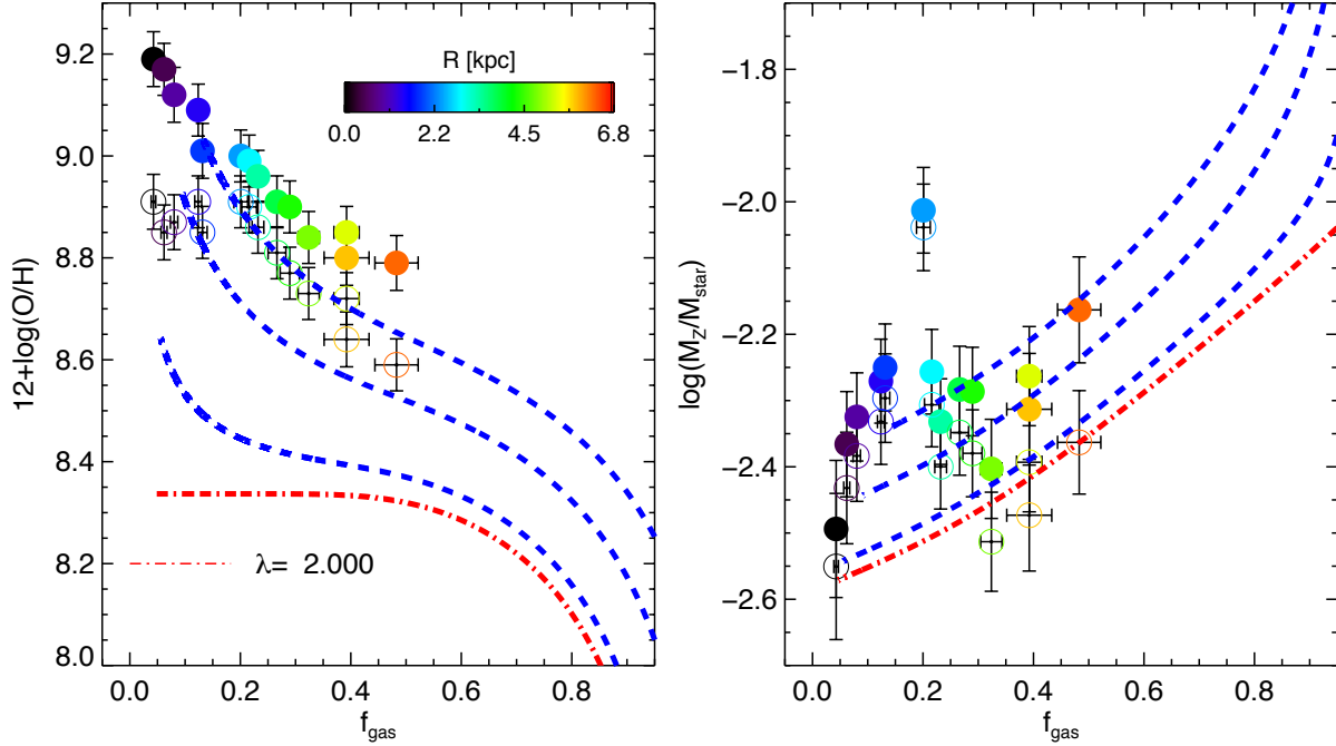
Figure 8. Same as Fig. 6 and 7, but including a late time inflow of gas rich material with metallicity 3 Z_{\odot} . The red line is the same as in Fig. 6 and 7 and represents the model with \lambda = 2 , while the blue lines represent an increasing mass of infalling metal-rich gas. Going upwards in both figures the blue lines represent an infalling metal-rich gas mass that is a fraction of 1%, 5% and 10% of the mass of baryons already present in the disc at a given location.
