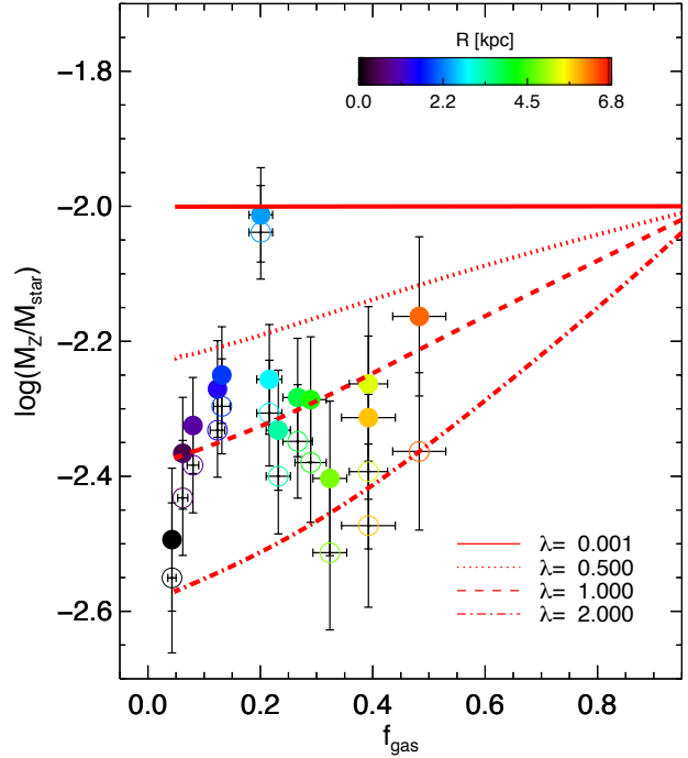
Figure 6. Metals-to-stellar mass ratio ( M_Z/M_\star ) versus gas fraction ( f_{\text{gas}} ). Symbols show the values observed in radial annuli in NGC628, where the colour-coding gives the galactocentric radial distance, as indicated in the colour bar. Solid symbols correspond to the mass of metals in which the ISM metallicity is calculated by using the M08 calibration, while open symbols use the PP04 calibration. The red lines correspond to the prediction of simple chemical evolution models with different values for the average outflow loading factor \lambda . Note that the model relations are independent of the inflow rate \Phi and of the star formation efficiency \varepsilon .
