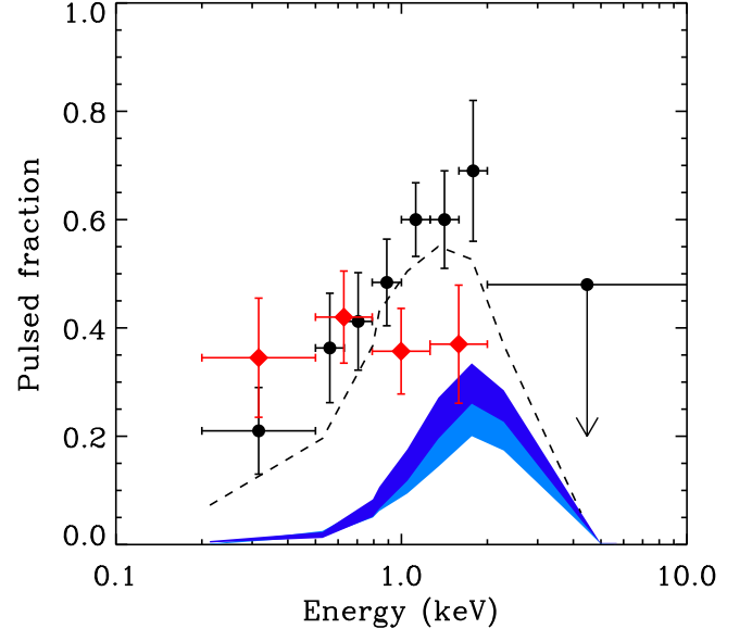
Figure 3. Pulsed fraction as a function of energy for the Q-mode (black dots) and B-mode (red diamonds) as derived from the 3D-ML analysis. Error bars are at 1\sigma , the upper limit at 2\sigma . The blue regions indicate the comparison with model atmosphere predictions for the most likely geometry of PSR B0943+10 (see Section 4.3). The dashed line is the pulsed fraction computed by Storch et al. (2014), corrected to account for the unpulsed non-thermal emission.
