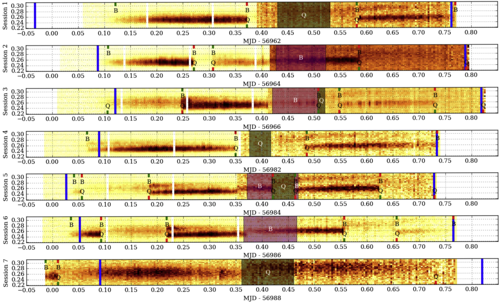
Figure 8. Summary of the LOFAR, LWA, and Arecibo radio data of the seven XMM-Newton observing sessions.
