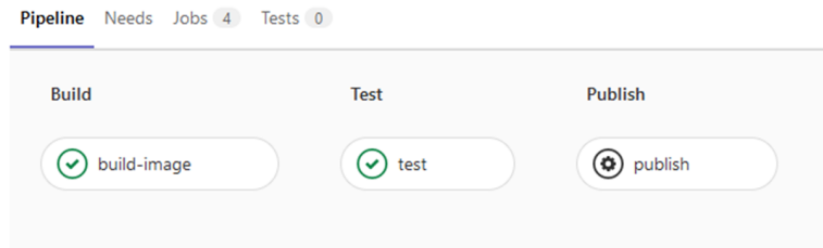
Figure 7. Gitlab Pipeline.
