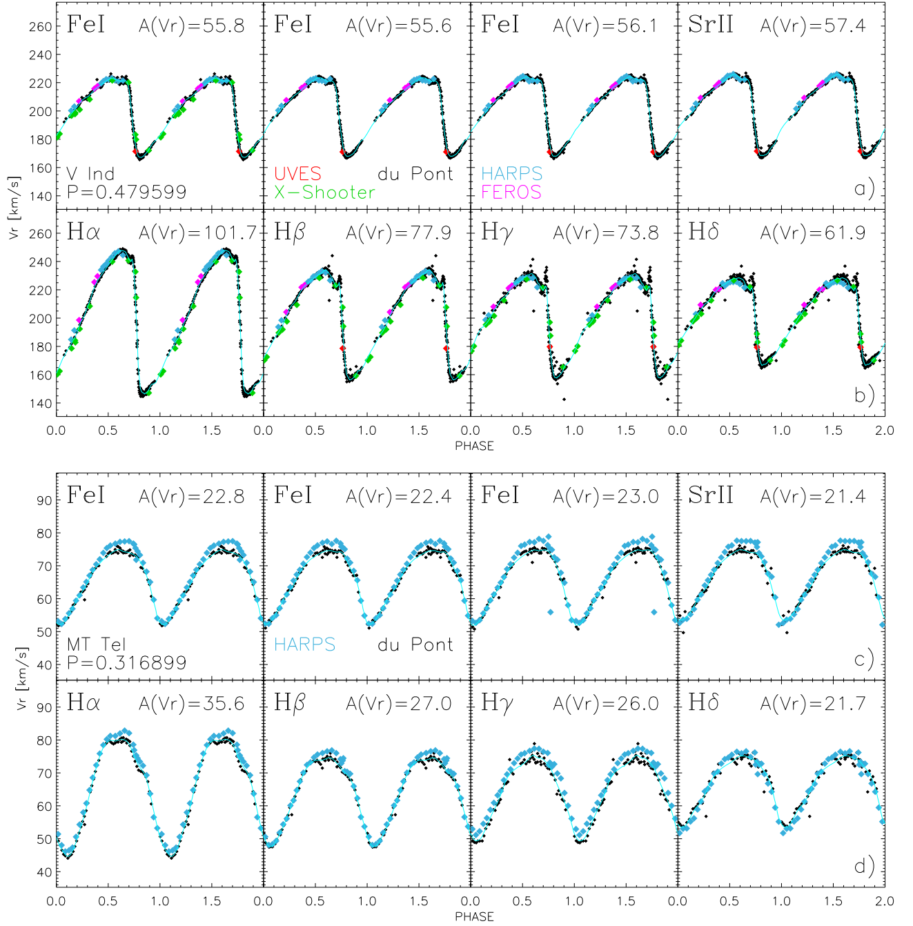
Figure 1. Panels a) and b): Radial velocity curves versus phase for the RRab V Ind based on metallic lines Fe I ( \lambda: 4045.81, 4063.59, 4071.74 \text{ \AA} ) and Sr II ( \lambda: 4077.71 \text{ \AA} ), and on Balmer ( \lambda: 6562.80, 4861.36, 4340.46, 4101.74 \text{ \AA} ) lines. Measurements based on different spectrographs are marked with different colors. The cyan lines show the analytical fits. The RV amplitude ( A(v_r) \text{km s}^{-1} ) and the pulsation period (days) are also labeled. Panels c) and d): Same as the top, but for the RRC MT Tel.
