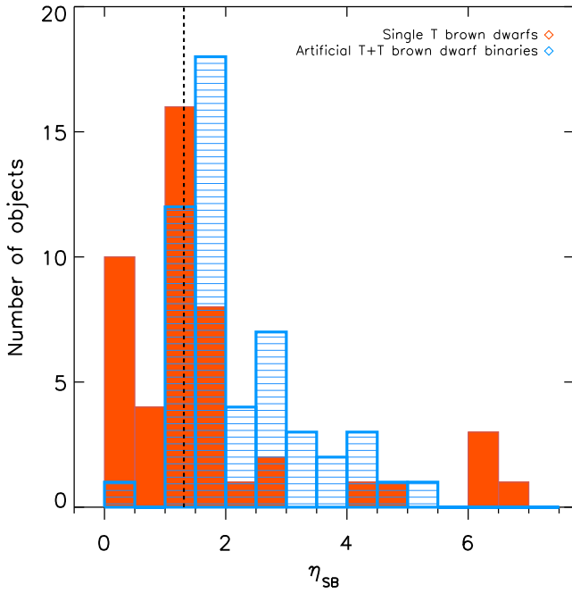
Figure 6. Histograms of \eta_{\text{SB}} for comparisons of single T brown dwarfs (in red) and artificial T plus T binaries (blue with lines), to other single T dwarfs and other T plus T synthetic binaries. The dashed black line indicates \eta_{\text{SB}} = 1.31 .
