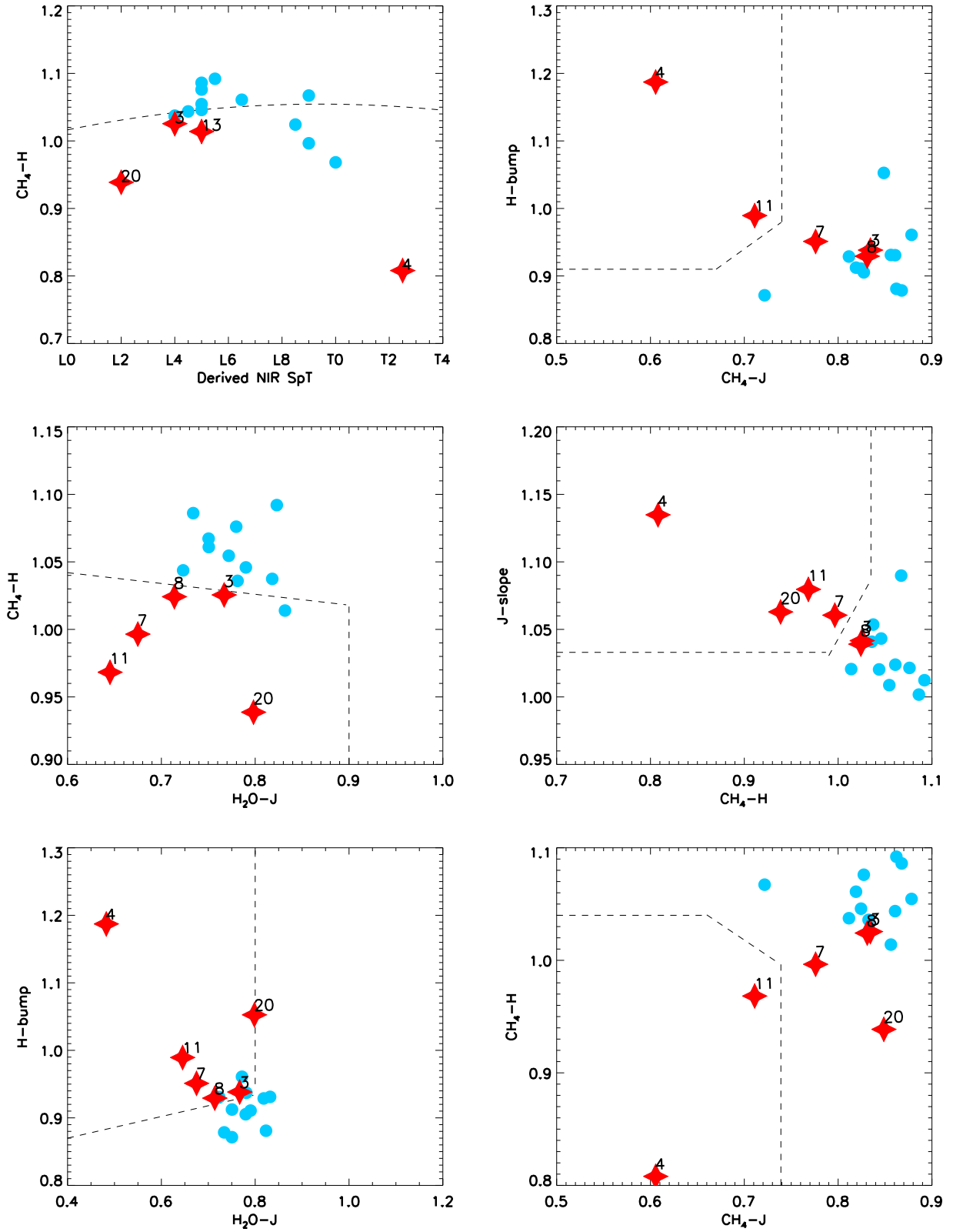
Figure C2. Spectral index selection.
