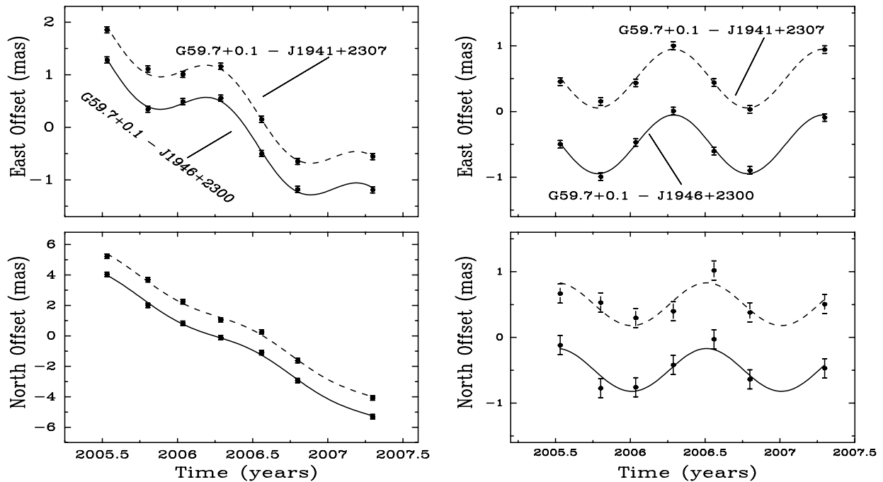
Figure 2. Position versus time for the reference maser spot at V_{LSR} 27.4 \text{ km s}^{-1} relative to two background radio sources (offset for clarity). The left and right panels indicate the positions of the maser spot before and after removing the fitted proper motion. The top and bottom panels show the eastward and northward offsets.
