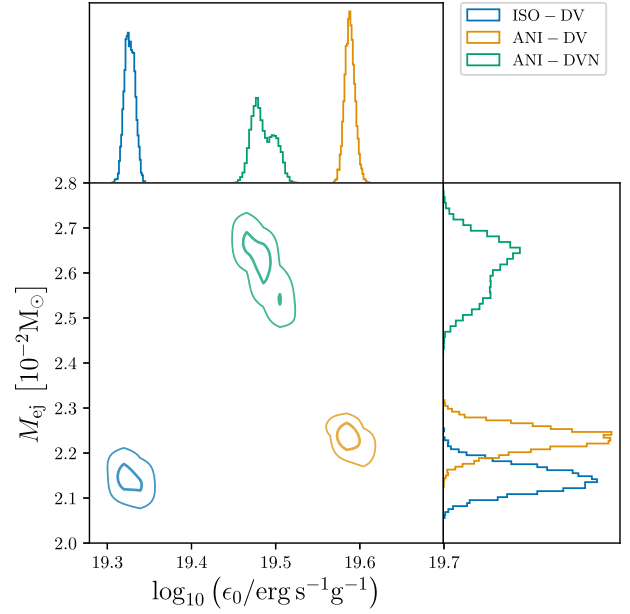
Figure 7. Marginalized posterior distribution of heating parameter \epsilon_0 and total ejected mass M_{\text{ej}} for three selected cases: ISO-DV (blue), ANI-DV (yellow), and ANI-DVN (green). The heating parameter \epsilon_0 is plotted using the logarithm to base 10 in order to evince the recovered orders of magnitude. The total mass M_{\text{ej}} is computed extending the sum to all the involved components.
