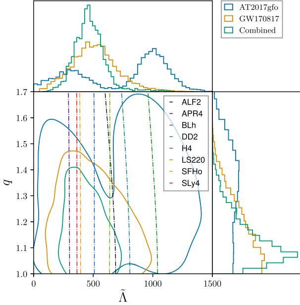
Figure 8. Posterior distribution in the (\tilde{\Lambda}, q) plane. The blue solid lines refer to the resampled values extracted from the k\text{N} analysis ( \text{ANI-DVN} ). The orange solid lines refer to the GW results, where the samples have been reweighted over a flat prior in \tilde{\Lambda} . The green solid lines are the combined inference. The contours represent the 90 per cent credible regions. The plot shows the expectations of some representative EOS.
