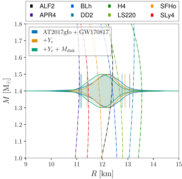
Figure 9. Posterior distribution of the radius R_{1.4} estimated with the joined inference of AT2017gfo and GW170817 plotted on top of the mass–radius relations coming from a sample of nuclear EOS (dashed lines). The blue solid line is computed using the mass and velocity information of the dynamical component, the orange solid curve takes into account also the contribution of the electron fraction, and the green solid line is the result with the additional inclusion of the disc mass information.
