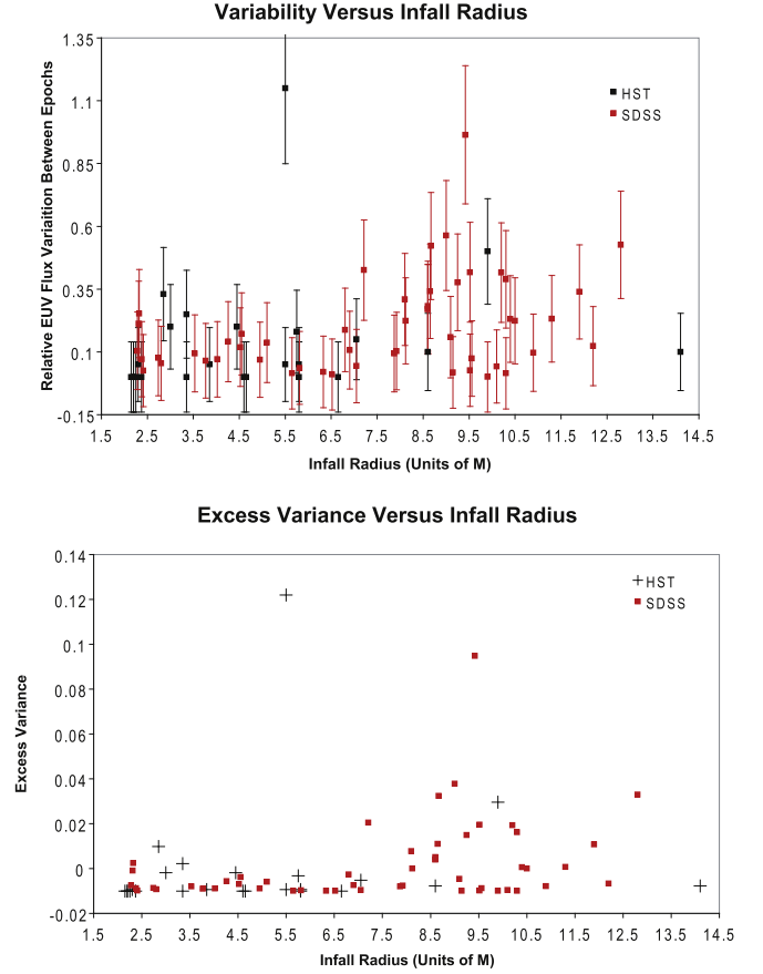
Figure 9. The top frame plots the relative variability vs. the infall radius from Tables 2 and 3. This infall radius is computed for the slim disk parameters that are given in Tables 2 and 3 by equating the infall time of the optically thin surface layer at that radius with the time between observations. The bottom frame is a plot of excess variance vs. infall radius. These plots give another crude measure of the location of the variable EUV emission. We find that significant variability starts to occur at a value of r \approx 7 M - 8.5 M in both plots for our fiducial model, consistent with the location of the EUV emitting region in Figure 6.
