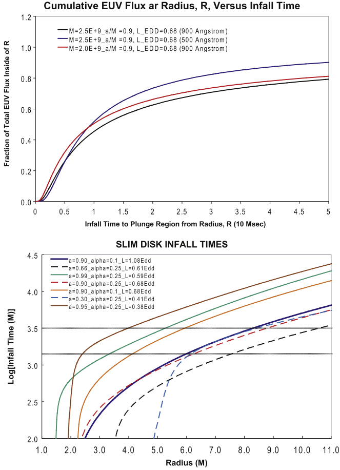
Figure 8. The top frame shows a plot of the fraction of the cumulative 900 Å flux density inside of a radius, R , F_{\lambda}(\lambda = 900 \text{ Å})|_{r < R} vs. the infall time from a radius, R , T_{\text{infall}}(R) based on the radial velocities that are calculated as in Figure 7. This indicates that the infall time from the EUV emitting region is a viable source of the timescale for EUV variability. The bottom frame plots the infall time (to a point mid way between the event horizon and the inner edge of the accretion disk) as a function of start radius for the trajectory. This is computed for the same slim disk parameters as were used in Figure 7. The horizontal dashed lines correspond to time intervals associated with variability that were shown in the right-hand side of Figure 2.
