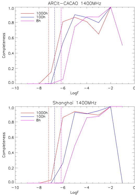
Figure 8. Completeness as a function of depth for the ARCIt-CACAO (top) and Shanghai (bottom) teams at 1.4 GHz. The vertical dotted lines are the 1\sigma noise RMS.
