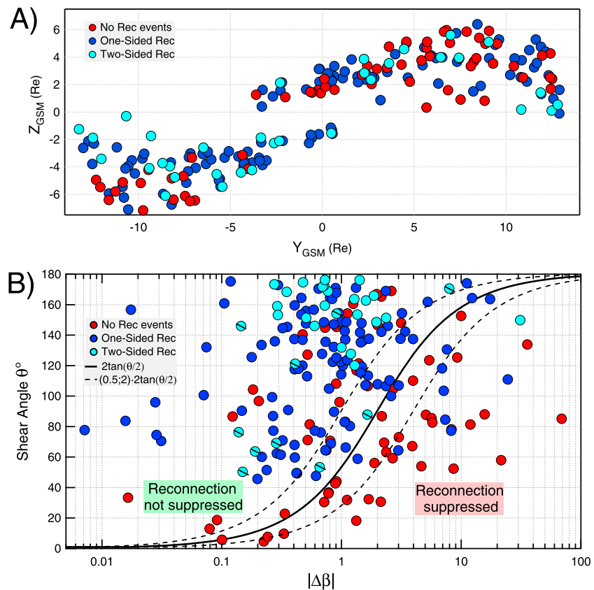
Figure 2. (a) The positions of the nonreconnection events (red dots), one-sided reconnection events (blue dots), and two-sided reconnection events (cyan dots) in the Y - Z_{GSM} plane. (b) The magnetic shear angle ( \theta ) as a function of |\Delta\beta| for the nonreconnection events (red dots), one-sided reconnection events (blue dots), and two-sided reconnection events (cyan dots). The black lines are the prediction for the diamagnetic suppression of reconnection (equation (1)), when \frac{L_p}{d_i} is equal to 1 (continuous line) or 0.5 or 2 (dashed lines). On the right of these curves, reconnection should be suppressed by diamagnetic drift effect, while on the left it should not be suppressed.
