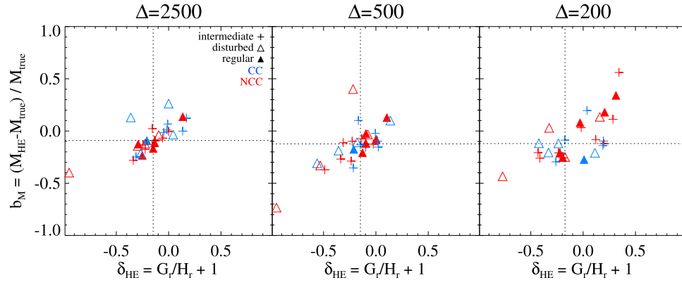
Figure 10. Relation between mass bias ( b_M ) and deviation from HE ( \delta_{HE} ), calculated at R_{2500} (left), R_{500} (middle), and R_{200} (right). In each panel, median values of the distributions are indicated by the dotted lines.
