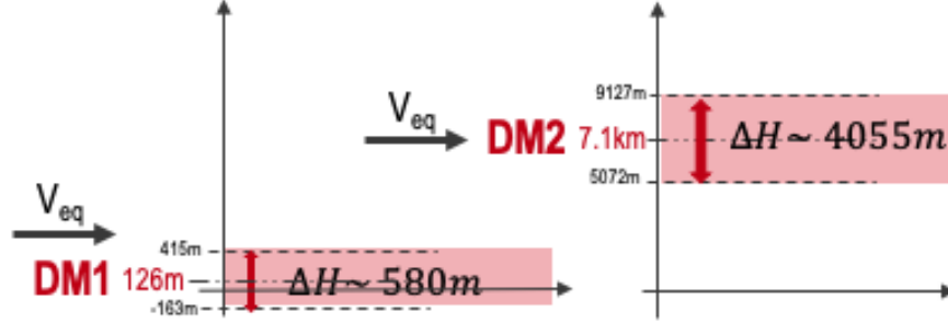
Figure 74: Vertical slabs of the atmosphere at which LINC-NIRVANA is sensitive to. Left: DM1. Right: DM2.
