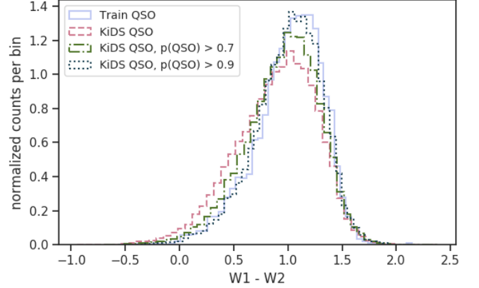
Fig. 11. Distribution of the mid-infrared W1-W2 color ( 3.4\mu\text{m} – 4.6\mu\text{m} , Vega) of quasar candidates in our KiDS sample, derived from a cross-match with all-sky WISE data. We show histograms for all KiDS QSOs matched with WISE, as well as for two examples of the probability cut: p_{\text{QSO}} > 0.7 , which is recommended to increase the purity of the sample, and p_{\text{QSO}} > 0.9 to illustrate how the resulting W1-W2 changes when the minimum probability considerably increases.
