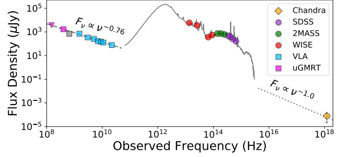
Fig. 3. Broadband radio to X-ray spectral energy distribution of FRB 2021124A. We show the best fit models to the radio (Appendix D), optical and infrared (Appendix F), and X-ray data (Appendix B) in gray. The dotted line represents the X-ray spectrum expected from the star formation derived from the optical SED modeling. It is dominated by a population of HMXB with a spectrum \approx \nu^{-1} (Fragos et al. 2013). The downward magenta triangle represents the uGMRT upper limit at 200 MHz. The gray square represents the uGMRT data at 650 MHz published by Wharton et al. (2021a).
