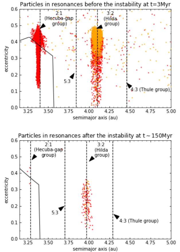
Fig. 21. In the top plot is shown the resonant groups after the early inward migration of the giant planets at t = 3 Myr. Vertical dashed lines indicate roughly the positions of the resonances and the solid black line delimits the asteroid belt region. In the bottom plot, we show the fate of the resonant populations after the instability of the giant planets with a characteristic time scale of \tau = 0.5 Myr, at t \sim 150 Myr. The resonance positions and the asteroid belt region are shifted in the bottom plot because Jupiter migrated from 5.4 to 5.2 au.
