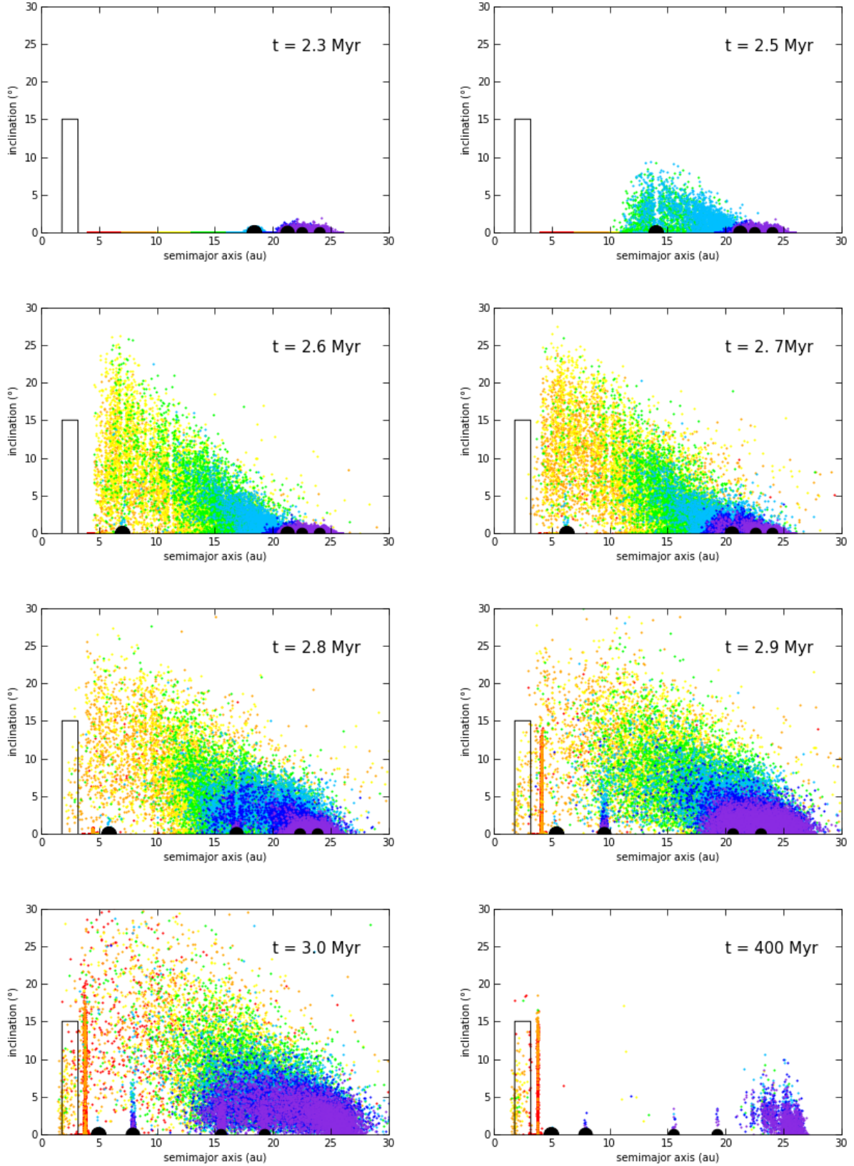
Fig. 5. As Figure 4, eight time-snapshots of inclination versus semimajor axis of one of the nominal model simulations are shown. The black line roughly delimits the main belt region. At t = 2.31 Myr, t = 2.56 Myr, t = 2.70 Myr and t = 2.70 Myr, Jupiter, Saturn, Uranus and Neptune (black filled dots) start to grow and to migrate inward and stop at t = 3 Myr. A fraction of bodies that were initially placed between 4 and 16 au, are injected in the asteroid belt region. Trojan asteroids are captured in the feeding zone of the planets' cores and carried along during the migration. As can be noted, particles grouped in the resonance 3:2 (the Hilda asteroids at roughly 4 au), gain their inclination because of Saturn migrating towards Jupiter. A small population of centaurs orbits between Jupiter and Neptune.
