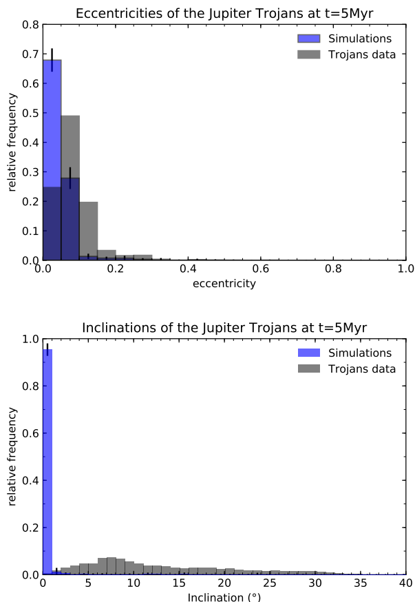
Fig. 9. Jupiter’s Trojans osculating eccentricities (top figure) and inclinations (bottom figure) at t = 5 Myr in the nominal model simulations are shown as blue histograms. The overplotted grey histograms represent the distribution of eccentricities and inclinations of the Jupiter Trojans in the MPC database.
