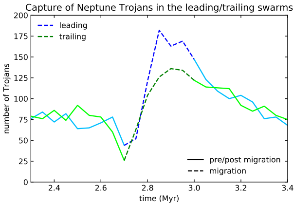
Fig. 14. The plot shows the number of particles in the leading and trailing side of the horseshoe orbits during the nominal model migration and growth of Neptune. The blue line is the number of particles in the L_4 side of the horseshoe orbit (leading side) versus time and the green line is the number of particles in the L_5 side of the horseshoe orbit (trailing side) versus time. We can clearly see an excess of leading particles during the growth and migration due to the deformations of the horseshoe orbit, but Neptune has not grown enough to shrink the orbits to stable tadpole orbits in order to preserve the asymmetry. Then when the migration stops the excess simply disappears because the horseshoe orbits are back symmetric. Dashed lines indicate the time frame where Neptune is growing and migrating.
