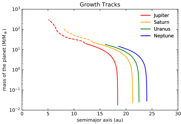
Fig. 1. The plot shows growth tracks for our nominal model. Jupiter (red line), Saturn (orange line), Uranus (green line) and Neptune (blue line) grow and migrate through the disc ending up in a more compact configuration compared to the current one. The solid lines indicate the core accretion phase, the dashed lines indicate the gas accretion phase.
