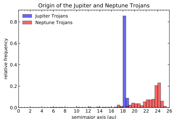
Fig. 10. Jupiter Trojans (blue histogram) and Neptune trojans (red histogram) origin in the nominal model simulations. Almost all the Jupiter Trojans are captured in the formation region of Jupiter’s core at about a \sim 18 au. Neptune Trojans are mainly particles from Neptune’s core feeding zone, but also particles scattered because of the earlier growth of Jupiter and Saturn.
