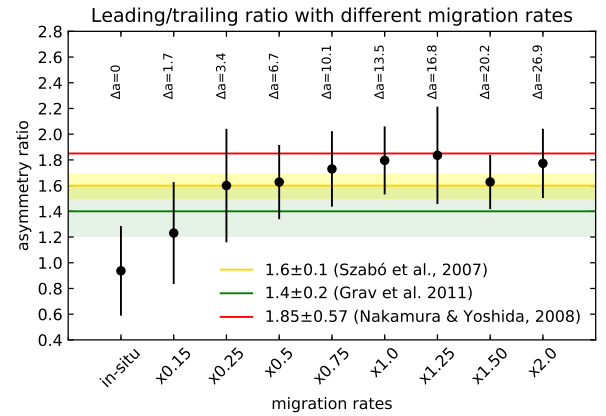
Fig. 8. The plot shows the asymmetry ratio, at t = 5 Myr, for different migration rates of the giant planets, plus the in situ scenario. The yellow shaded region highlights the observed asymmetry ratio of 1.6 \pm 0.1 found by Szabó et al. (2007) and the green shaded region represents the observed asymmetry ratio of 1.4 \pm 0.2 found by Grav et al. (2011). The red line indicates the estimated asymmetry ratio of 1.85 \pm 0.57 found by Nakamura & Yoshida (2008). In this latter case the shaded region has not been overplotted to keep the figure readable, but the uncertainty is indicated in the legend. Above each asymmetry ratio it is noted the corresponding migration \Delta a that Jupiter undergoes.
