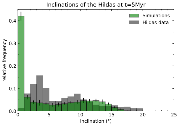
Fig. 15. Osculating eccentricities (top figure) and inclinations (bottom figure) of the Hilda asteroids at t = 5 Myr with Jupiter and Saturn that end locked in the 1:2 resonance.
