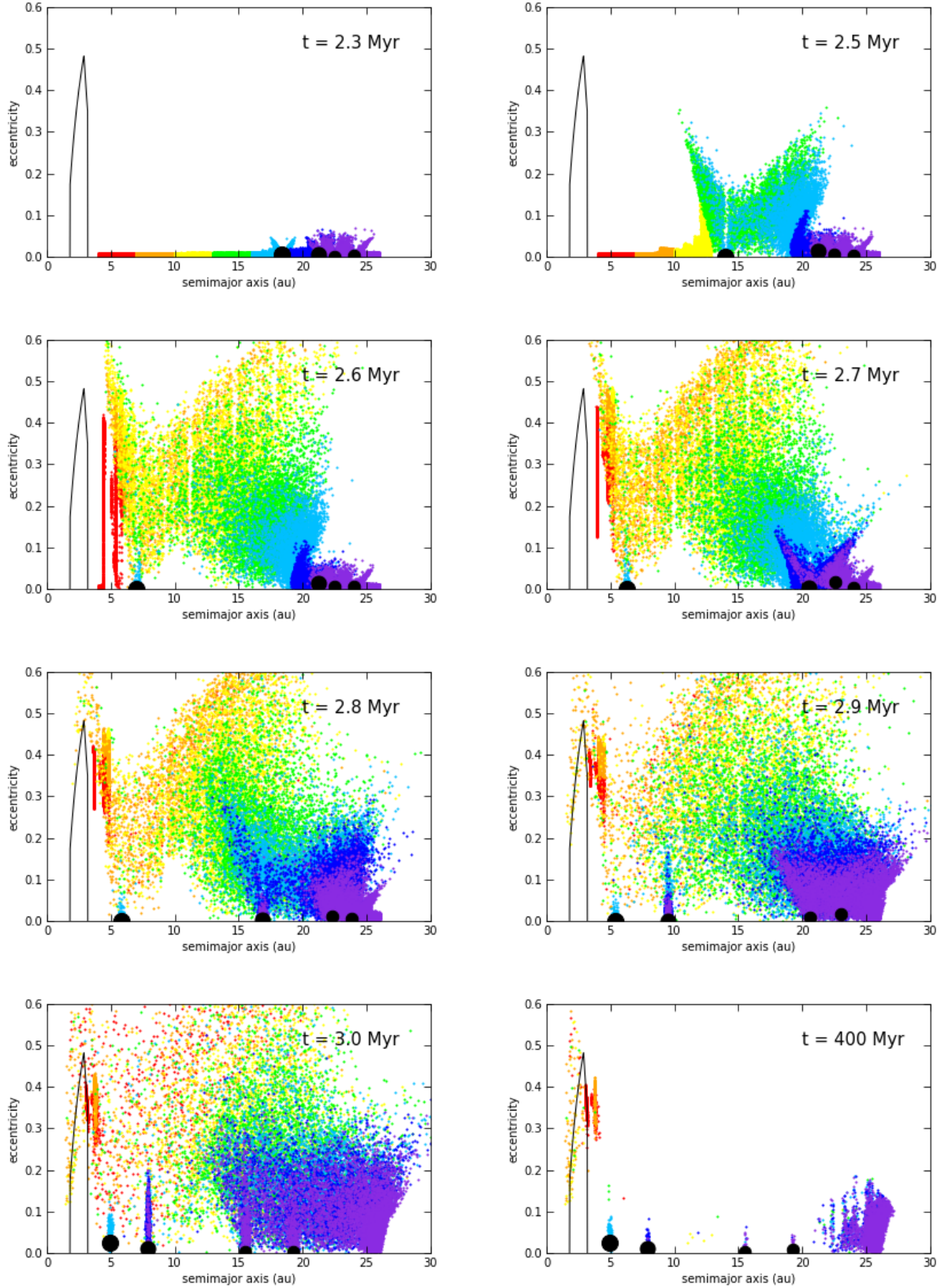
Fig. 4. The figure shows eight time-snapshots of eccentricity versus semimajor axis of one of the nominal model simulations. The black line roughly delimits the main belt region. At t = 2.31 Myr, t = 2.56 Myr, t = 2.70 Myr and t = 2.70 Myr, Jupiter, Saturn, Uranus and Neptune (black filled dots) start to grow and to migrate inward and stop at t = 3 Myr. A fraction of bodies that were initially placed between 4 and 16 au, are injected in the asteroid belt or possess enough eccentricity to cross the terrestrial planet region. Trojan asteroids are captured in the feeding zone of the planets' cores and carried along during the migration. Each of the four planets captured Trojans, but, after t = 400 Myr, Saturn's, Uranus' and Neptune's are drastically reduced because of planetary interactions. Particles clump in the resonance 3:2 (the Hilda asteroids at roughly 4 au) and other populated resonances are shown in Figure 6. A small population of centaurs orbits between Jupiter and Neptune.
