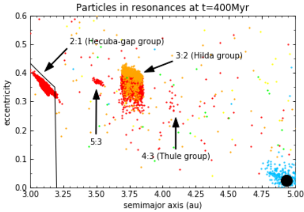
Fig. 6. Zoom in of the region between 3 and 5 au in figure 4. It is possible to distinguish different resonant populations. From the left to the right in the plot: the Hecuba-gap group in the 2:1 mean motion resonance with Jupiter (3-3.25 au); a population in the second order 5:3 resonance with Jupiter (3.5 au); the Hilda asteroids in the 3:2 mean motion resonance with Jupiter (3.75 au); the Thule group in the 4:3 resonance (4.1 au). The black line roughly delimits the main belt region. We note that in this nominal case, due to interactions with the other planets, the final semimajor axis of Jupiter is about 5 au and the location of the resonances are slightly shifted inward.
