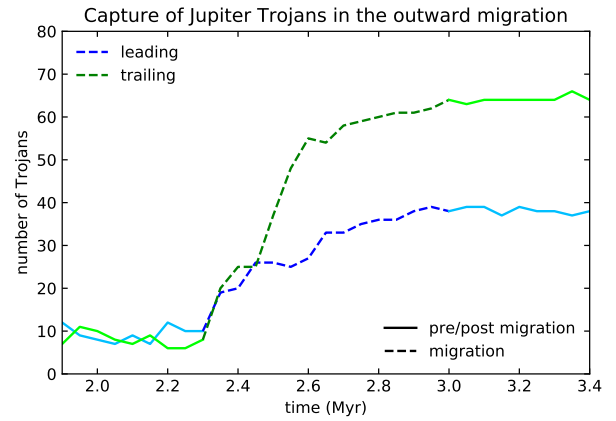
Fig. 12. The plot shows the number of particles in the leading and trailing side of the horseshoe orbits during the outward migration and growth of Jupiter from 5 au to 18 au. The blue line is the number of particles in the L_4 side of the horseshoe orbit (leading side) versus time and the green line is the number of particles in the L_5 side of the horseshoe orbit (trailing side) versus time. As expected, in the case of outward migration, particles spend more time in the trailing part of the orbit, because the path of the particles is wider on that side. Dashed lines indicate the time frame where Jupiter is growing and migrating.
