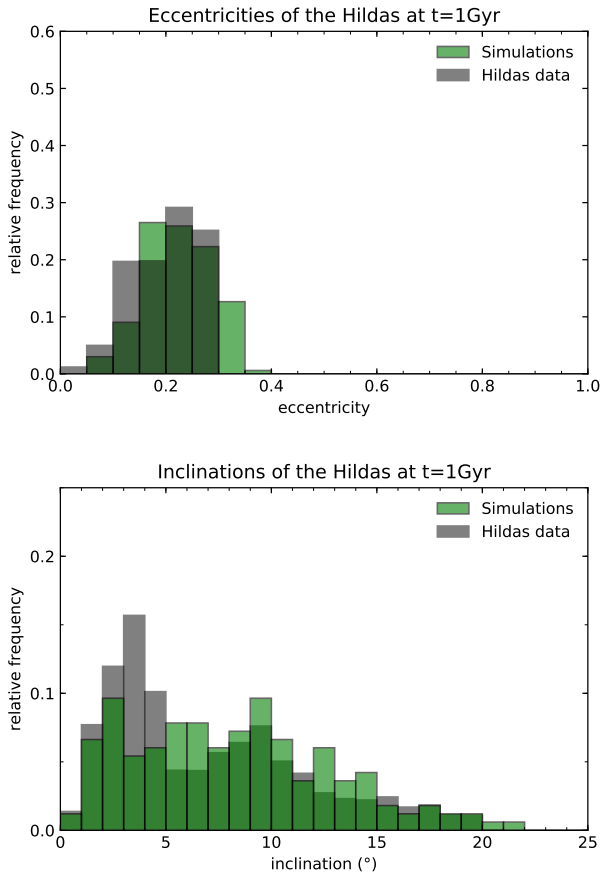
Fig. 20. Osculating eccentricities (top figure) and inclinations (bottom figure) of the Hilda asteroids at t = 1 Gyr in a model where Jupiter and Saturn, after their growth and early migration where they ended up in the 2:1 resonance, subsequently migrate to their final orbits on a characteristic time scale of \tau = 0.5 Myr.
