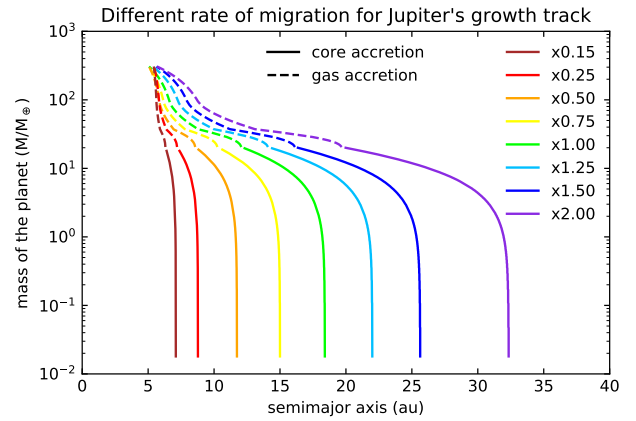
Fig. 3. Different rates of migration for Jupiter growth tracks compared to the nominal migration rate (green line). The brown, red, orange and yellow curves are associated with slower migration rates: 0.15, 0.25, 0.50 and 0.75 times the nominal rate of migration, respectively. The blue, dark blue and violet curves are associated with faster migration rates: 1.25, 1.50 and 2.00 times the nominal migration rate, respectively. The solid lines indicate the core accretion phase and the dashed lines indicate the gas accretion phase. Due to interactions between the gas giants during the migration, Jupiter does not exactly end up with the same semimajor axis for each migration rate.
