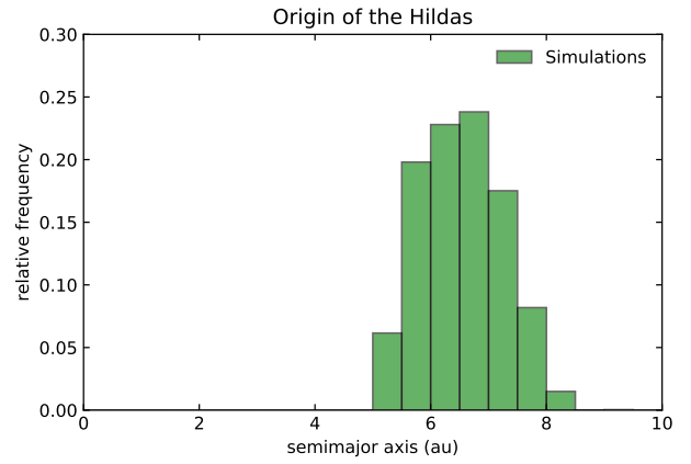
Fig. 17. Original formation regions of the bodies trapped in the 3:2 mean-motion resonance with Jupiter.
