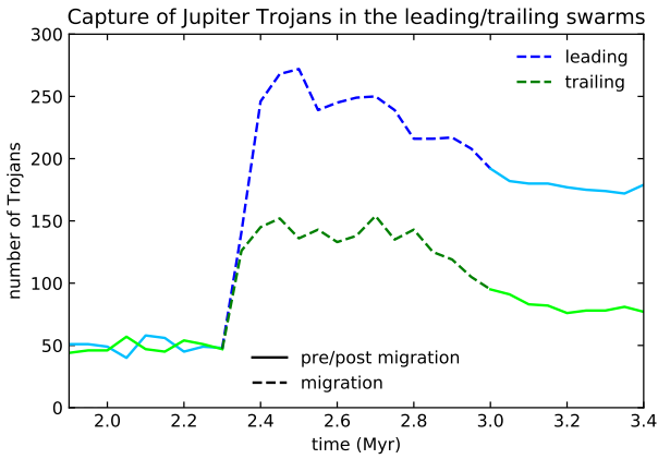
Fig. 11. The plot shows the number of particles in the leading and trailing side of the horseshoe orbits during the nominal model migration and growth of Jupiter. The blue line is the number of particles in the L_4 side of the horseshoe orbit (leading side) versus time and the green line is the number of particles in the L_5 side of the horseshoe orbit (trailing side) versus time. Horseshoe orbit encompass both L_4 and L_5 , hence an excess of leading particles means that particles spend more time in the leading part of the orbit. Dashed lines indicate the time frame where Jupiter is growing and migrating.
