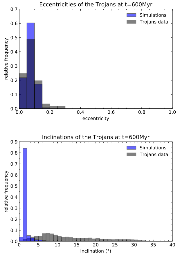
Fig. 19. Osculating eccentricities (top figure) and inclinations (bottom figure) of the Trojan asteroids at t = 600 Myr for \tau = 0.5 Myr when Jupiter and Saturn experience an instability after the disc disperses at t = 3 Myr.
