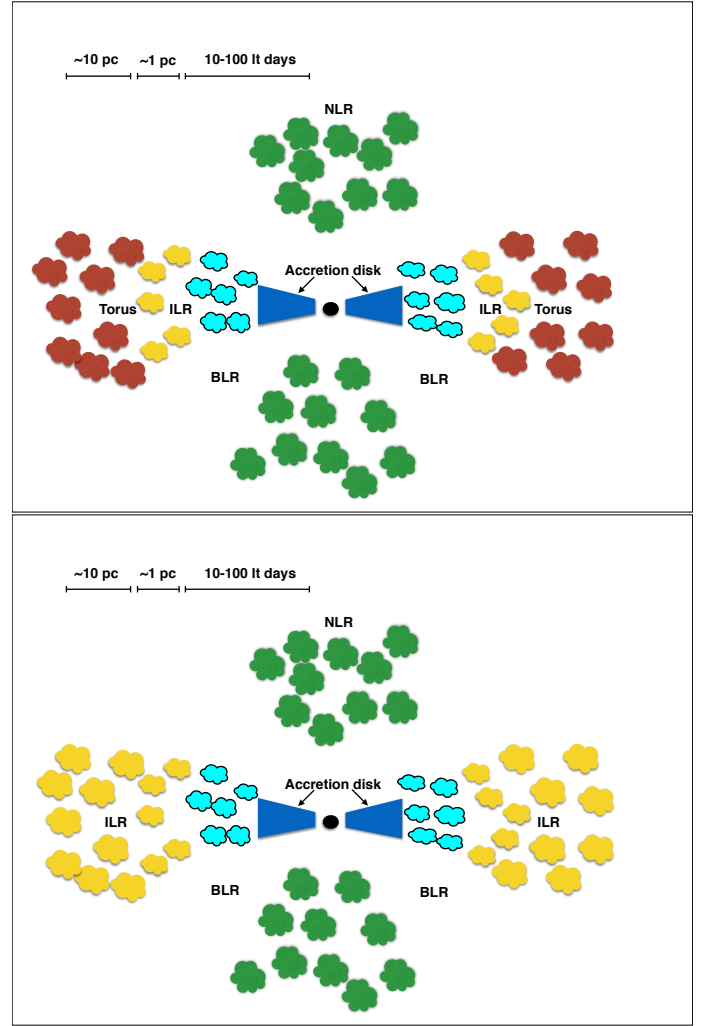
Fig. 9. Schematic view of the ILR in Seyfert galaxies ( top panel ) and LINER galaxies ( bottom panel ). The image is not on scale.
