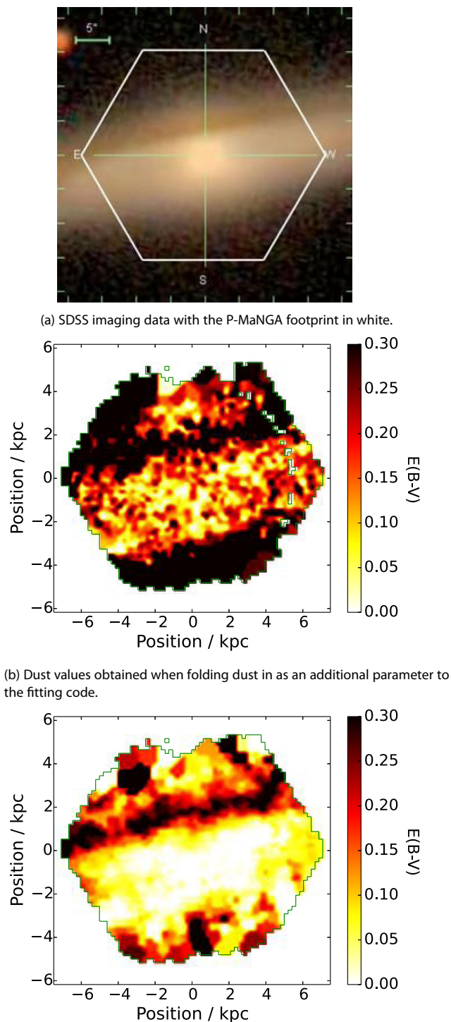
Figure 2. The effect of different methods for dealing with dust attenuation in fitting codes with the example galaxy p4-127A (in Table 2), analysed using MILES-based M11 models with its full parameter range.
