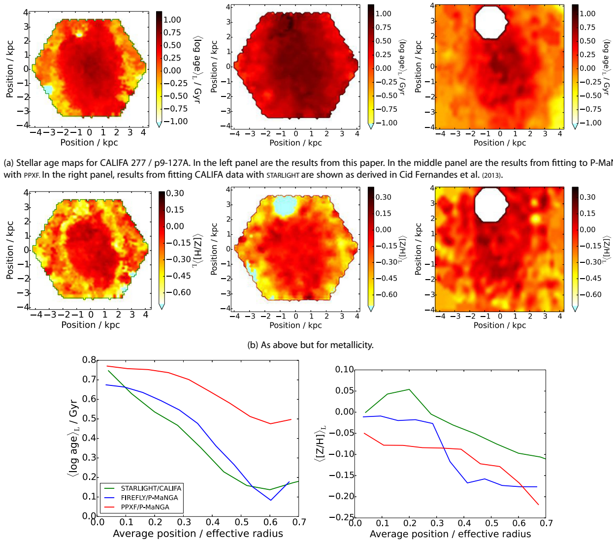
Figure 16. Derived stellar population maps and profiles for CALIFA-277, known in this paper as p9-127A, a target shared by both the P-MaNGA and CALIFA surveys at observational conditions similar to those expected for MaNGA. The galaxy as observed with CALIFA is analysed with the spectral fitting code STARLIGHT, and is compared to the results from P-MaNGA observations with both FIREFLY analysis and analysis with PPXF as described in Section 5.6.
