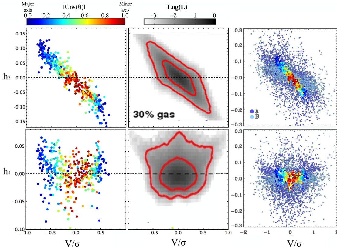
Figure 5. Left-hand panels: the h_3 - V/\sigma (top) and the h_4 - V/\sigma (bottom) distributions from the VIMOS kinematical maps. Points are colour-coded according to the azimuthal deviation from the galaxy minor axis. Middle panels: comparison with predictions from 1:1 disc-disc merger simulations from H+09 with 30 per cent gas fraction. The shading is proportional to the logarithm of the luminosity, whose scale is plotted in the bar on the top and the red contours contain 68 and 95 per cent of the luminosity. Right-hand panels: comparison with predictions of N+14 simulations for galaxies of class A and B.
