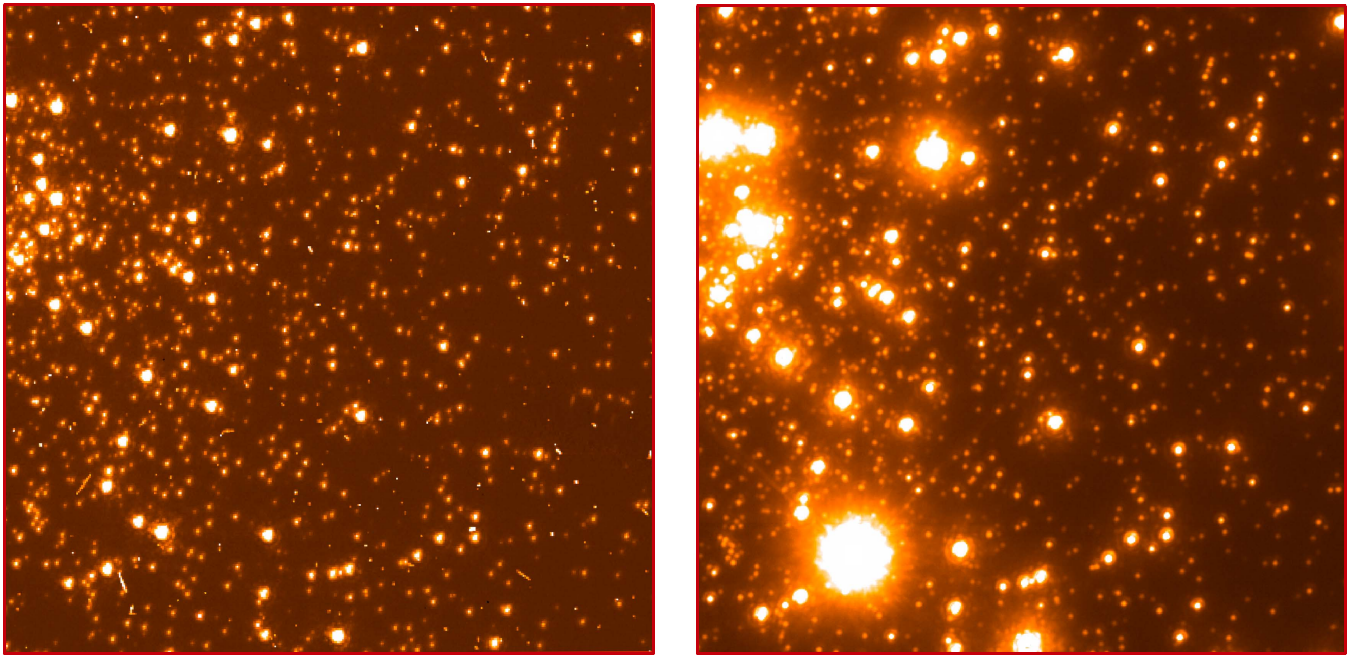
Figure 2. A zoom-in of a central region ( 10'' \times 10'' ) of the cluster as seen by ACS/HRC (F435W filter) on board HST (Dalessandro et al. 2014, left) and by GSAOI + GeMS in the K_s band (this work, right). The spatial resolution of GEMINI in the NIR turns out to be comparable to that of the HST in the optical.
