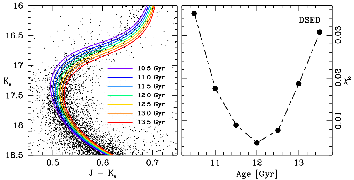
Figure 9. Same as in Figure 7, but for DSED isochrones.
