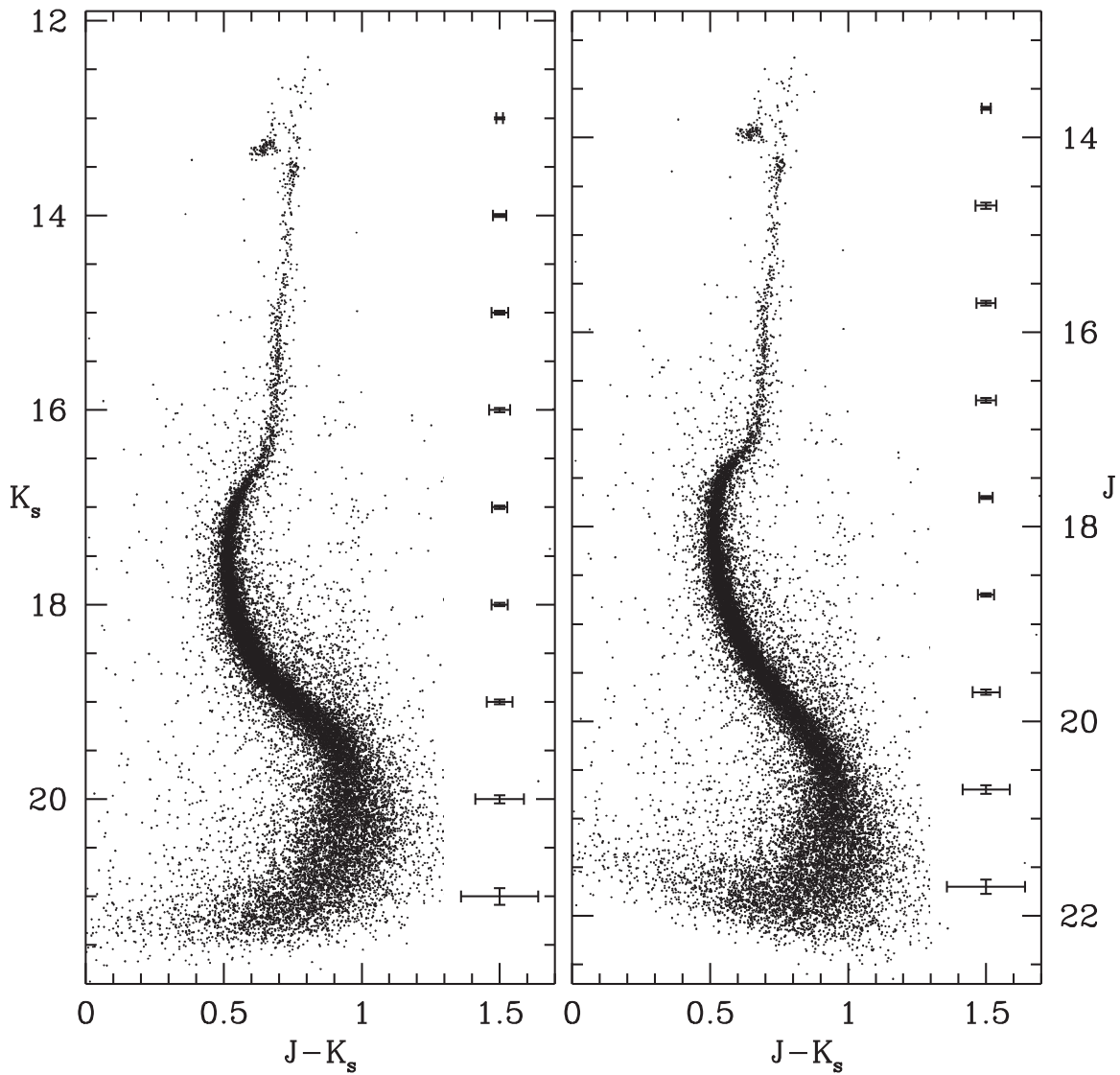
Figure 5. ( K_s , J - K_s ) and ( J , J - K_s ) CMDs of NGC 6624 obtained from the GEMINI observations discussed in the paper. All the main evolutionary sequences of the cluster are well visible, from the RGB, HB, MS-TO down to the MS-K. These NIR diagrams turn out to be comparable to the HST optical ones, both in depth and in photometric accuracy. The photometric errors for each bin of K_s and J magnitudes are shown on the right side of the panels.
