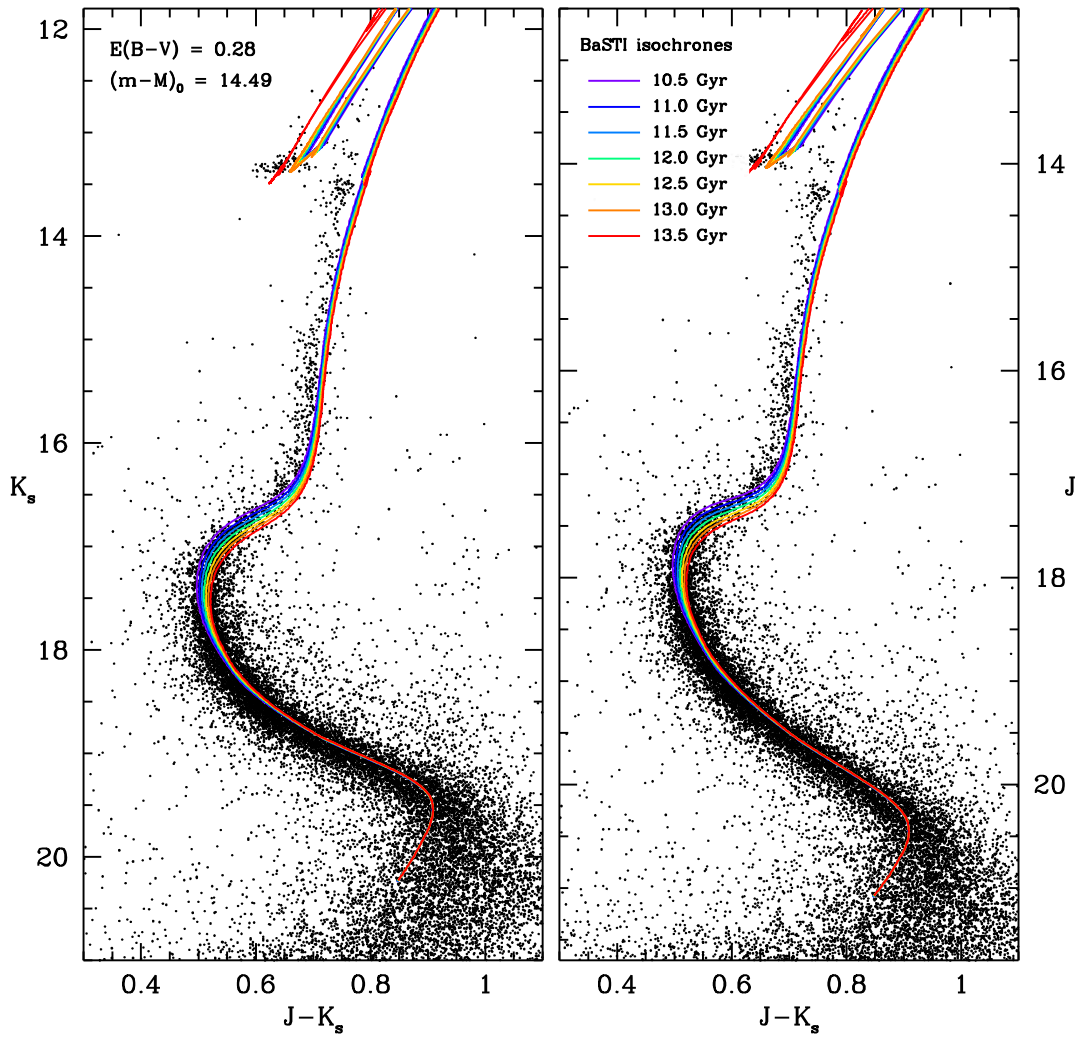
Figure 6. (K_s, J - K_s) and (J, J - K_s) CMDs of NGC 6624 CMDs with overplotted a set of BaSTI (Pietrinferni et al. 2004) isochrones with ages ranging from 10.5–13.5 Gyr, in steps of 0.5 Gyr (see labels).
