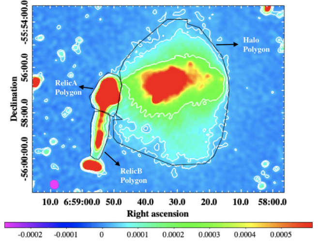
Figure 2. MeerKAT’s low resolution image of the diffuse emission. The rms of the image is 10.1 \mu\text{Jy beam}^{-1} . The beam, indicated by the magenta ellipse, has a size of 13.1 \text{ arcsec} \times 11.7 \text{ arcsec} and the position angle of the beam is 120.6^\circ . The black polygons indicate the regions that were used to calculate the flux density of the diffuse emission. The contour levels are [3, 6, 20] \times \sigma where \sigma = 10.1 \mu\text{Jy beam}^{-1} .
