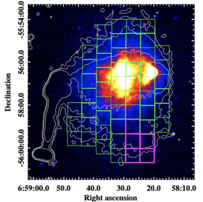
Figure 3. X-ray image of the Bullet cluster obtained from archival Chandra ACIS-I observations by Markevitch (2006). The overlaid contours are from MeerKAT's low resolution image. The contour levels are [3, 6, 20] \times \sigma where \sigma = 10.1 \mu\text{Jy beam}^{-1} . The beam size of the low resolution image is 13.1 \text{ arcsec} \times 11.7 \text{ arcsec} and the position angle of the beam is 120.6^\circ . The grid shows the region which was used to perform the point-to-point analysis. All the cells were used for the MeerKAT analysis, while the magenta cells were excluded for the ATCA analysis.
