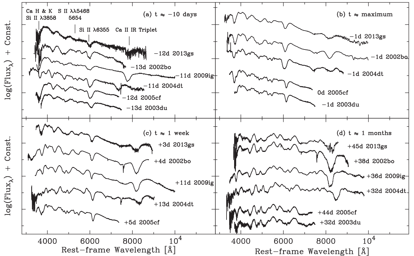
Figure 8. Spectra of SN 2013gs at four different epochs ((a)–(d), t \approx -12 days, -1 days, +3 days, and 1 months from B -band maximum), shown along with spectra of other SNe 2002bo, 2003du, 2004dt, 2005cf, and 2009ig at similar epochs (see the text for references). All spectra have been corrected for the redshift of host galaxy and shifted in the vertical direction for better display.
