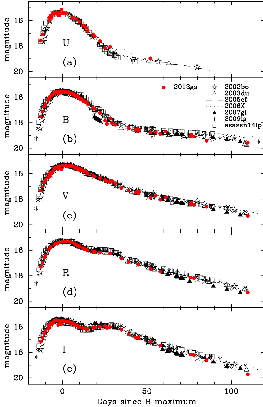
Figure 3. UBVRI light curves of SN 2013gs, and the comparison SNe 2002bo, 2003du, 2005cf, 2006X, 2007gi, 2009ig, and ASASSN-14lp (see the text for references). All light curves are shifted in magnitude to match the peak of SN 2013gs.
