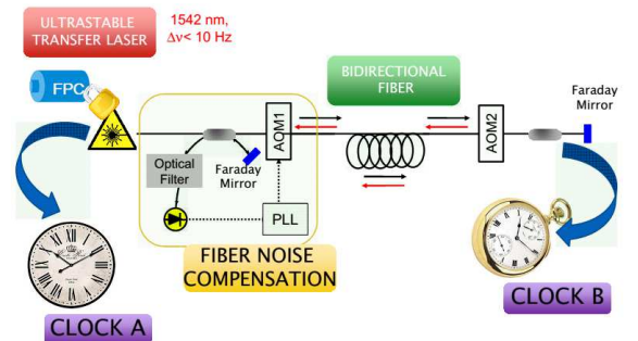
Fig. 3. Coherent optical fiber link: onceptual scheme.
