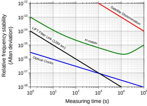
Fig. 2. Relative frequency Allan deviation of Hydrogen Masers, optical clocks and the transfer methods based on satellites or optical fibers.
