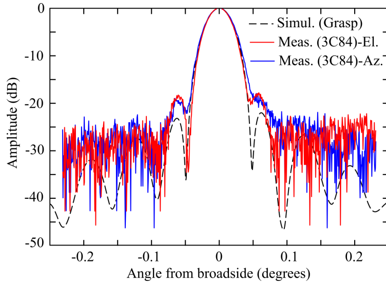
Figure 27: Normalized radiation pattern of the SDSA at 8.45 GHz: comparison between the GRASP simulation and the orthogonal (azimuthal and elevation) cuts measured by performing cross-scan of 0.5^\circ length on 3C84.
