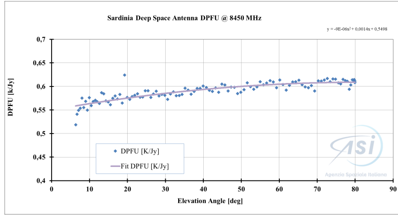
Figure 29: Antenna Gain Curve DPFU (degrees per flux density unit).
