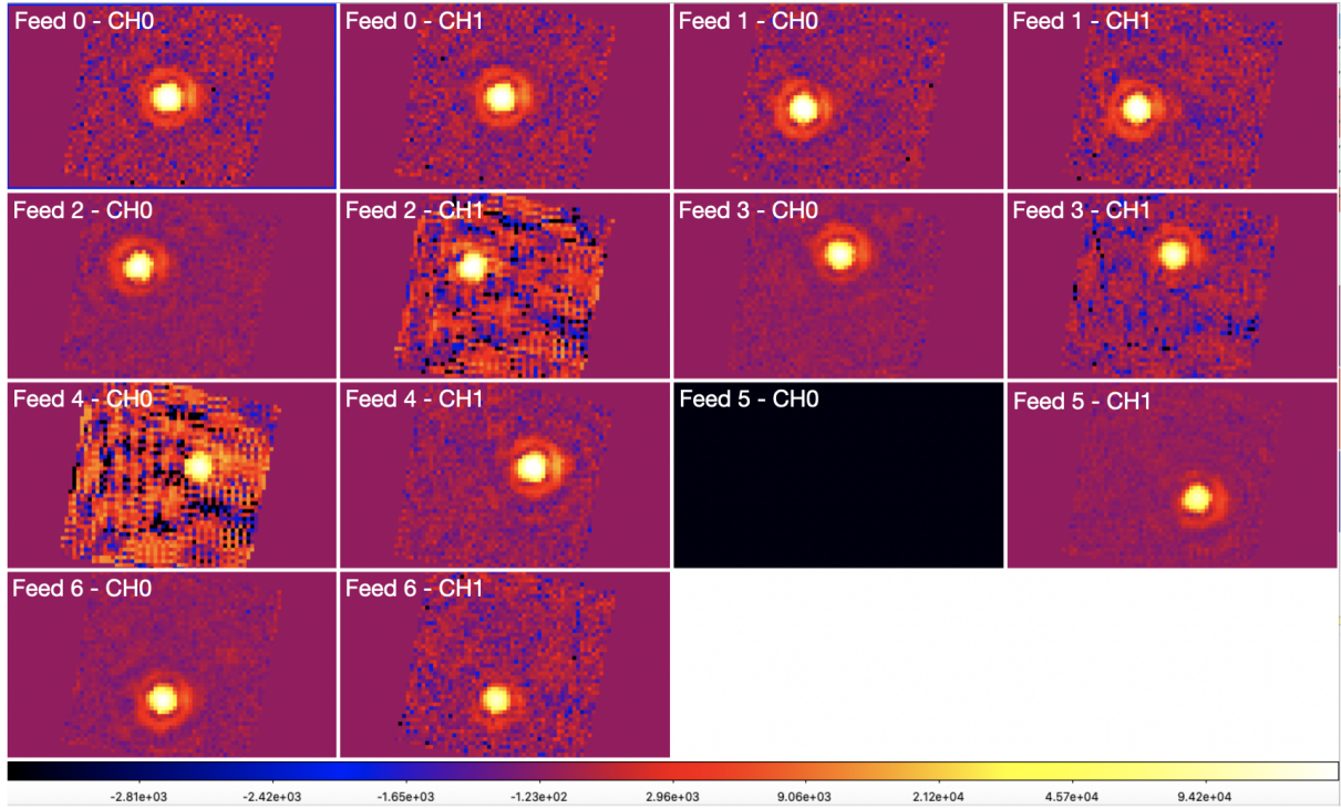
Figure 22: Maps of 3C84 ( 0.2^\circ \times 0.2^\circ ) obtained for Ch0 and Ch1 corresponding to the 7 feeds at 60^\circ \text{el} on 17/12/2020.
