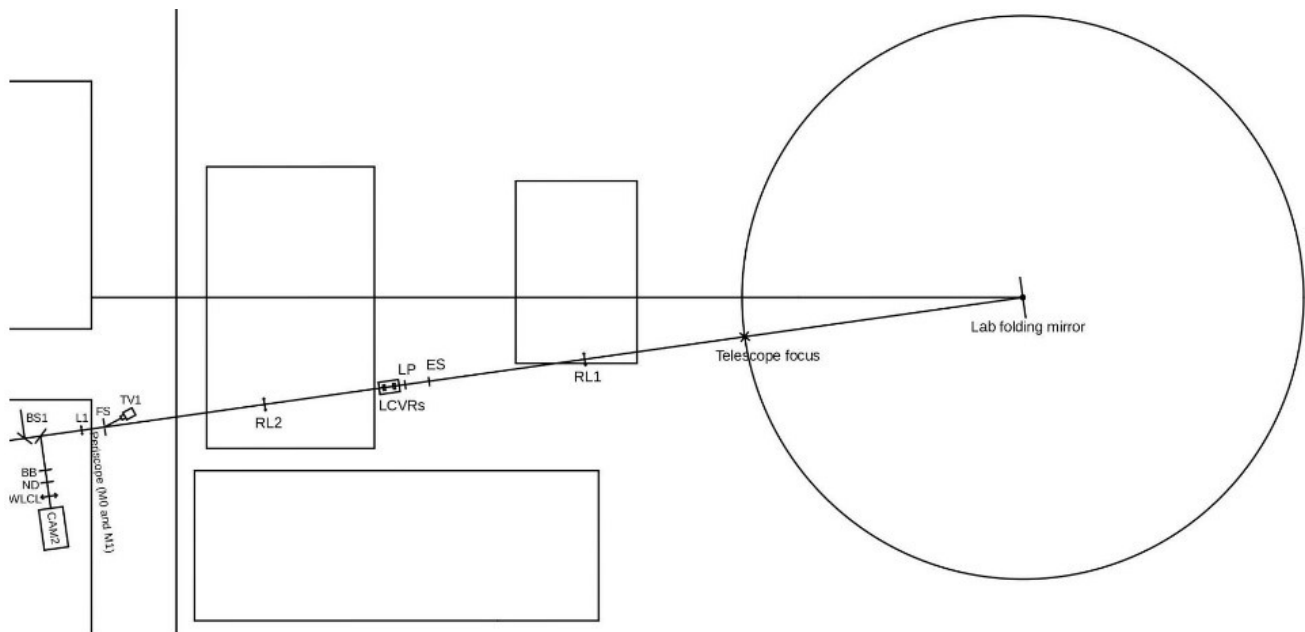
Figure 1. Optical relay system (RL1 and RL2) between the telescope focus at VTT and the IBIS 2.0 Field Stop (FS). The Entrance Shutter (ES) is placed in the pupil between the two relay lenses. The calibration Linear Polarizer (LP) and the two Liquid Crystal Variable Retarders (LCVRs), the modulator of the polarimeter, are placed \sim 150 mm after the pupil image on the ES. The rectangles show optical tables, the circle indicates the position of the telescope focus rotating with the Lab folding mirror.
