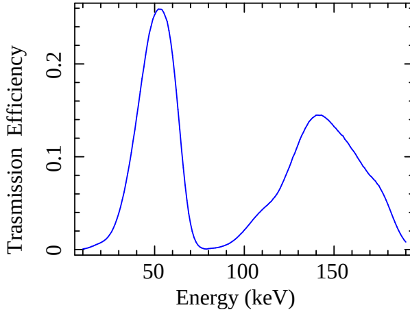
Fig. 3 Total transmission probability relative to the medium filter as function of the input proton energy. It accounts for the filter, the MOS electrode together with the factor for the fraction of events that are detected in the energy range 0.2-10 keV.
