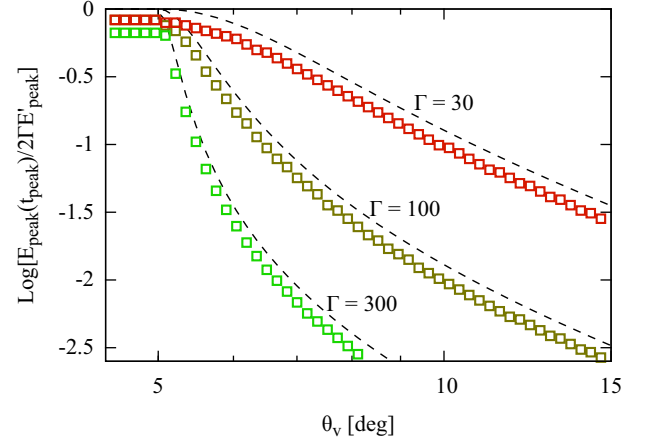
Figure 12. E_{\text{peak}} at the pulse peak time for three jets with R = 10^{13} cm, \theta_{\text{jet}} = 5^\circ and three values of \Gamma , namely (from red to green) \Gamma = 30, 100 and 300 . The black dashed lines are plots of \delta_B/2\Gamma for the corresponding values of \Gamma .
