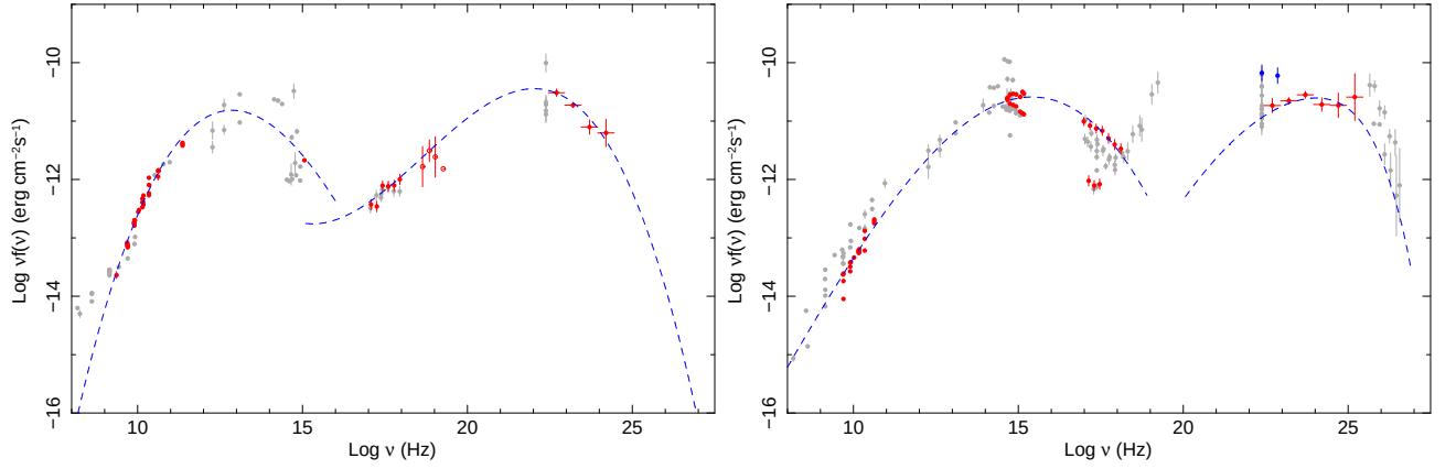
Fig. 14.— The SED of 0FGL J1159.2+2912 = 4C29.45 (left) and of 0FGL J1221.7+2814 = ON231 = W Comae (right)
