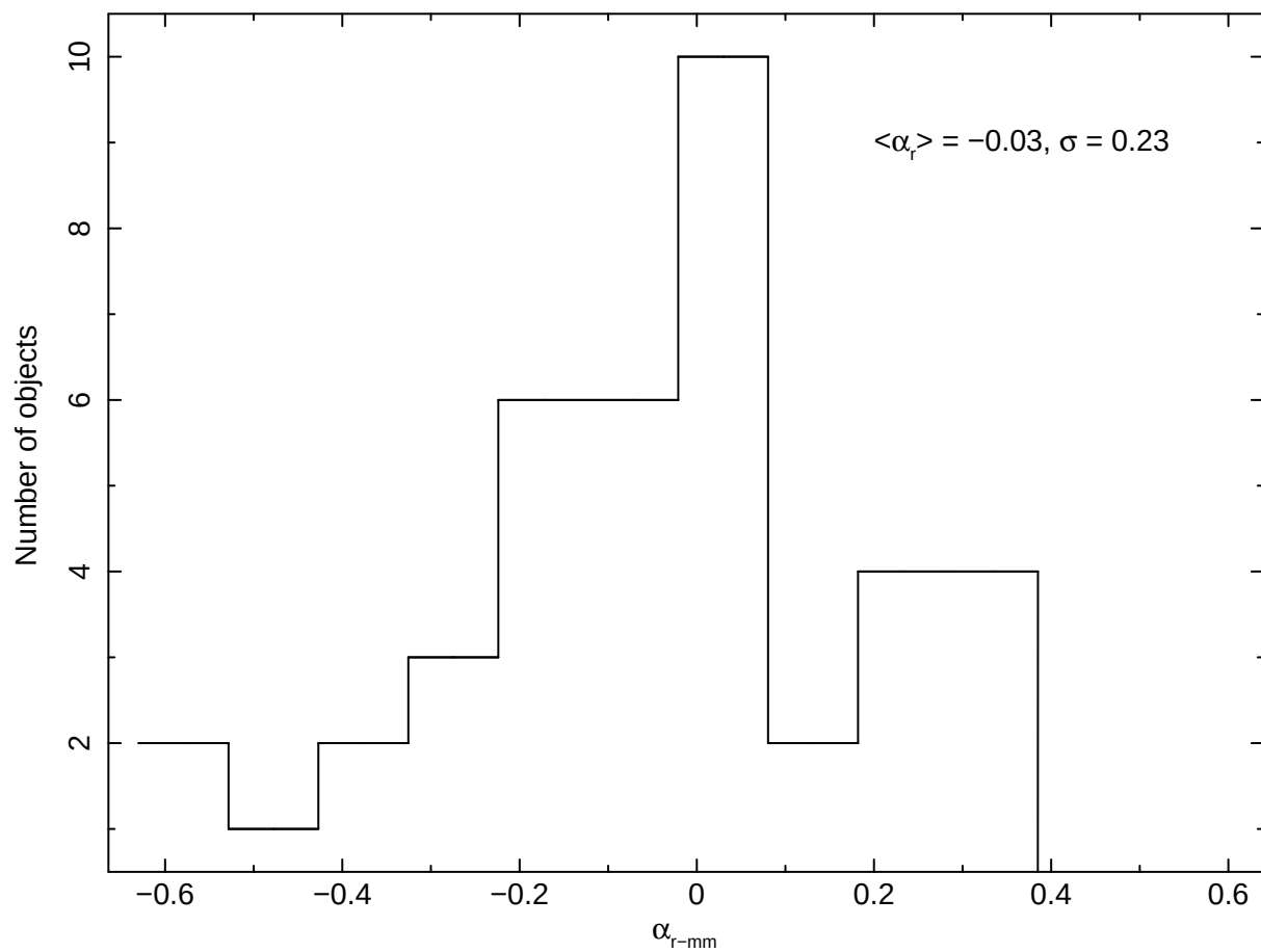
Fig. 25.— The distribution of radio spectral index ( f_r(\nu) \propto \nu^{\alpha_r} ) measured with the radio data of our 48 SEDs.
