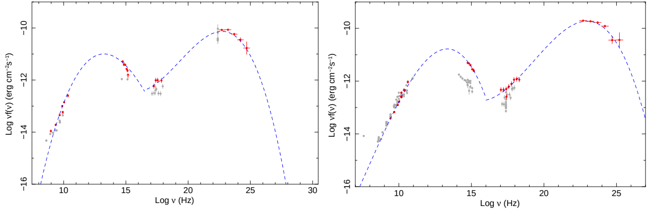
Fig. 17.— The SED of 0FGL J1457.6-3538 = PKS 1454-354 (left) and of 0FGL J1504.3+1030 = PKS1502+106 (right)
