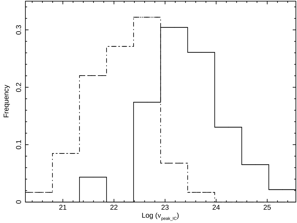
Fig. 33.— The distribution of inverse Compton peak frequency for the sample of LBAS FSRQ (dot-dashed line) and BL Lacs (solid line).
