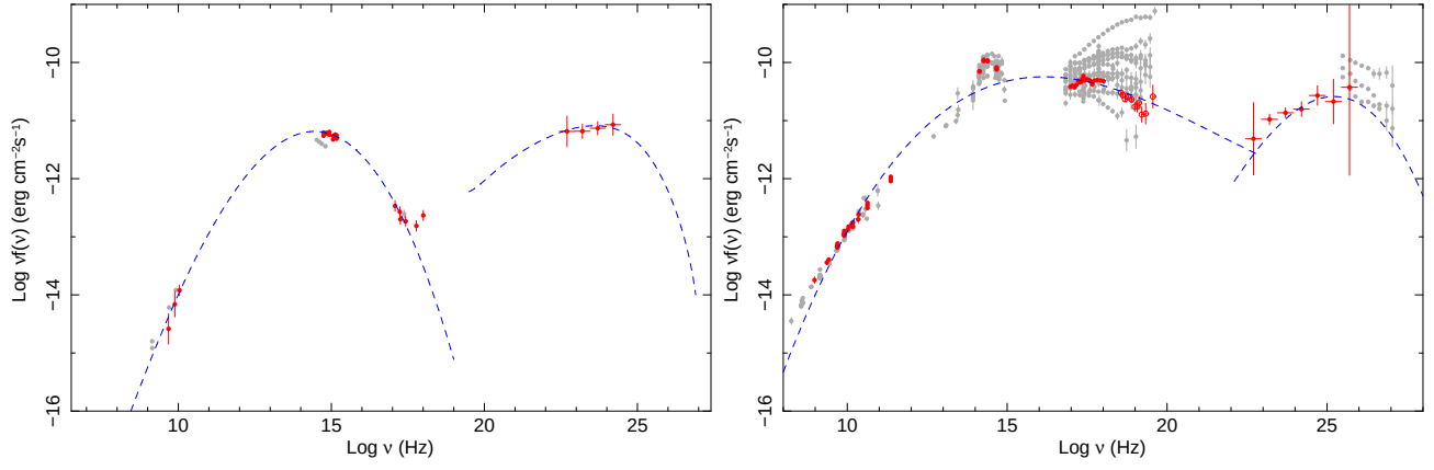
Fig. 19.— The SED of 0FGL J1543.1+6130 = GB6 J1542+6129 (left) and of 0FGL J1653.9+3946 = Mkn 501 (right)
