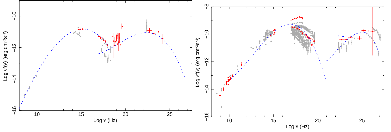
Fig. 13.— The SED of 0FGL J1058.9+5629 = GB6 J1058+5628 (left) and of 0FGL J1104.5+3811 = Mkn 421 (right)
