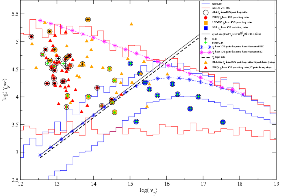
Fig. 36.— \gamma_{peak}^{SSC} obtained by Eq. 7 for the objects reported in Table 10. blue solid boxes represent HPB objects, orange solid boxes represent IPBs/LPBs objects and red solid circles represent FSRQs. The black solid line represents \nu_{peak}^S estimated by Eq. (6) for both the ERC and the SSC numerical SEDs, the blue solid line represents \gamma_{peak}^{SSC} estimated from Eq. (7) applied to numerically computed the SSC SEDs, and the solid purple line represents the same for the case of ERC emission. The true value of the simulation is represented by the black dashed line. Parameters of the model are given in Sect. 9. The blue and red contours delimit the area covered by the estimate of \gamma_{peak}^{SSC} for the case of SSC and ERC models respectively and for a Monte Carlo simulation with values of \delta ranging between 10 and 15, B ranging between 0.01 and 1G and T ranging between 10 and 10^{4.5} K.
