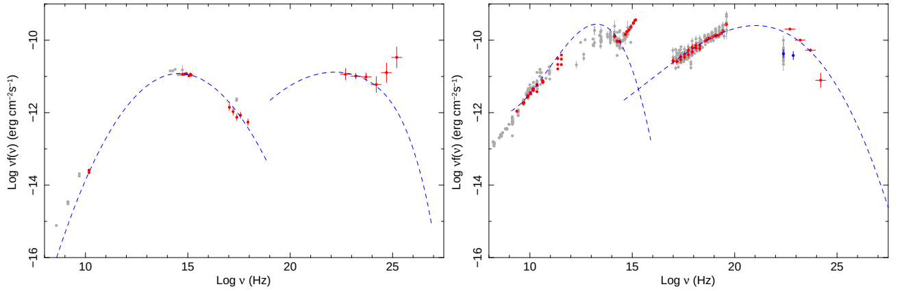
Fig. 15.— The SED of 0FGL J1248.7+5811 = PG 1246+586 (left) and of 0FGL J1229.1+0202 = 3C273 (right)
