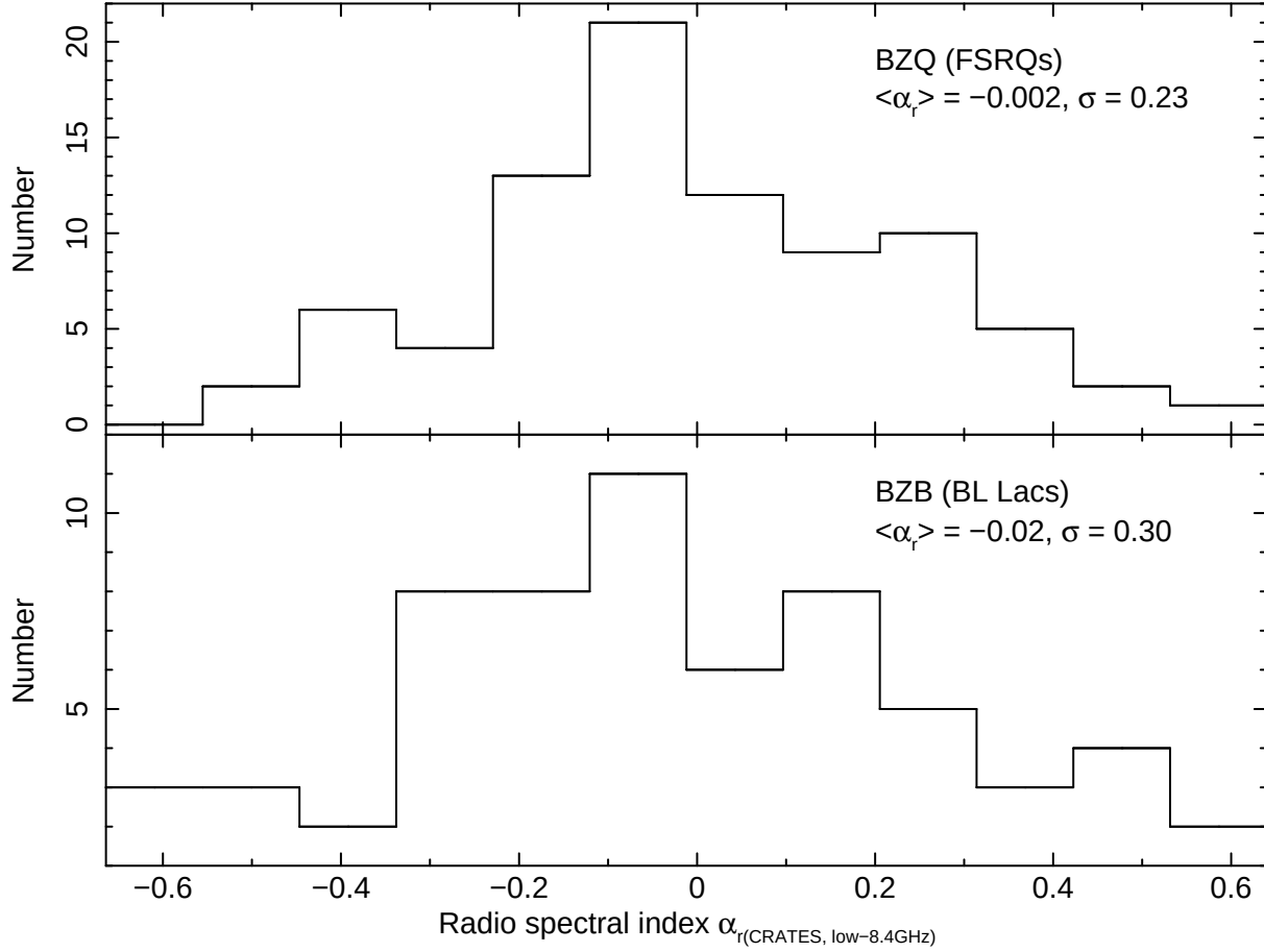
Fig. 26.— The distribution of radio spectral index ( f_r(\nu) \propto \nu^{\alpha_r} ) taken from the CRATES catalog, estimated between the CRATES low frequency, ( \sim 1\text{GHz} ) and 8.4 GHz, for the sample of FSRQ (top panel) and BL Lacs (bottom panel).
