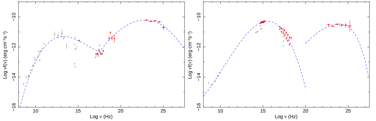
Fig. 6.— The SED of 0FGL J0428.7-3755 = PKS0426-380 (left) and of 0FGL J0449.7-4348 = PKS0447-439 (right)
