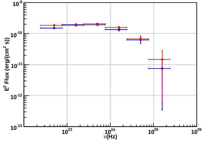
Fig. 38.— Comparison of the SEDs of the blazar ASO0235+164 obtained with the maximum likelihood approach (red points) and with the unfolding technique (blue points). The horizontal error bars represent the bin width.
