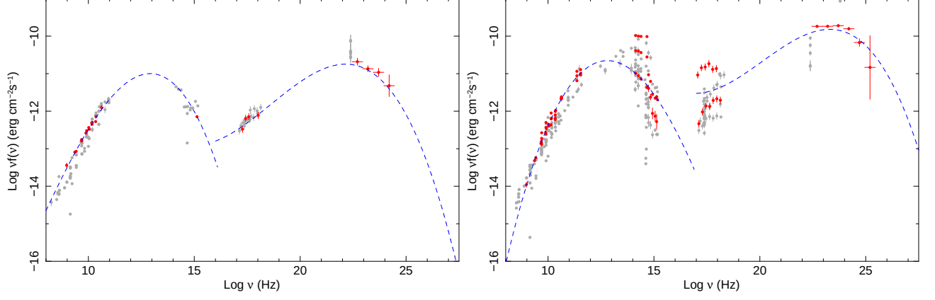
Fig. 4.— The SED of 0FGL J0238.4+2855 = 4C28.07 (left) and of 0FGL J0238.6+1636 = PKS0235+164 (right).
