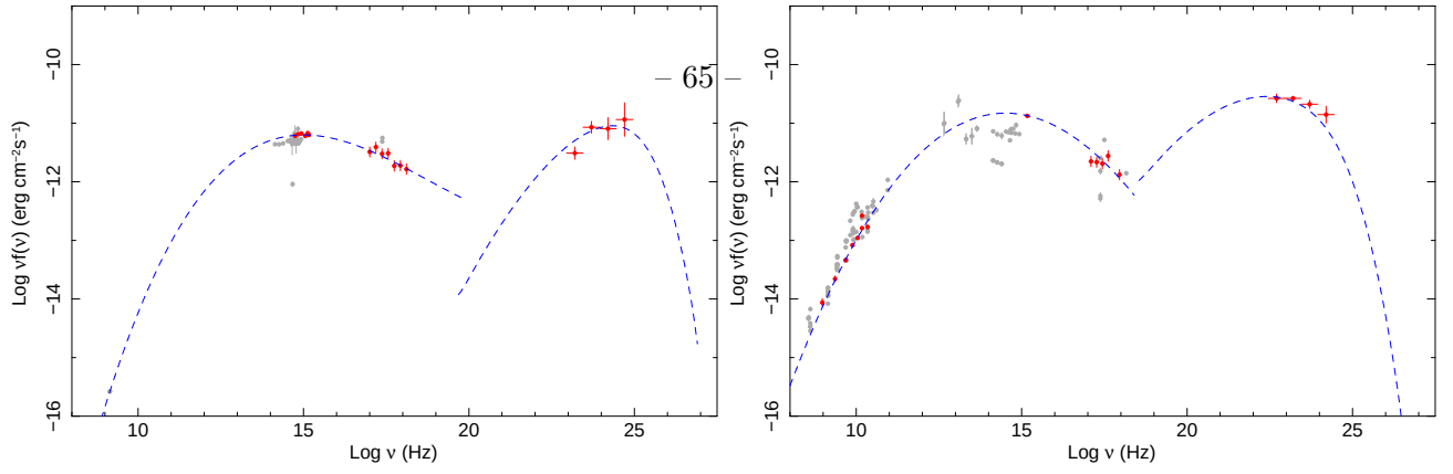
Fig. 1.— The SED of 0FGL J0033.6-1921 = 1RXS J003334.6-192130 = SHBL J003334.2-192133 (left) and of 0FGL J0050.5-0928 = PKS0048-09 (right). The quasi-simultaneous data appear as large filled red symbols, while non-simultaneous archival measurements are shown as small open grey points. The dashed lines represent the best fits to the Synchrotron and Inverse Compton part of the quasi-simultaneous SEDs (see text for detail).
