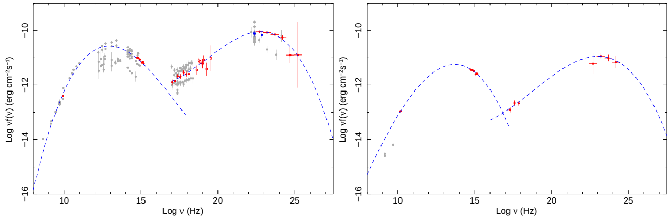
Fig. 9.— The SED of 0FGL J0538.8-4403 = PKS0537-441. (left) and of 0FGL J0712.9+5034 = GB6 J0712+5033 (right)
