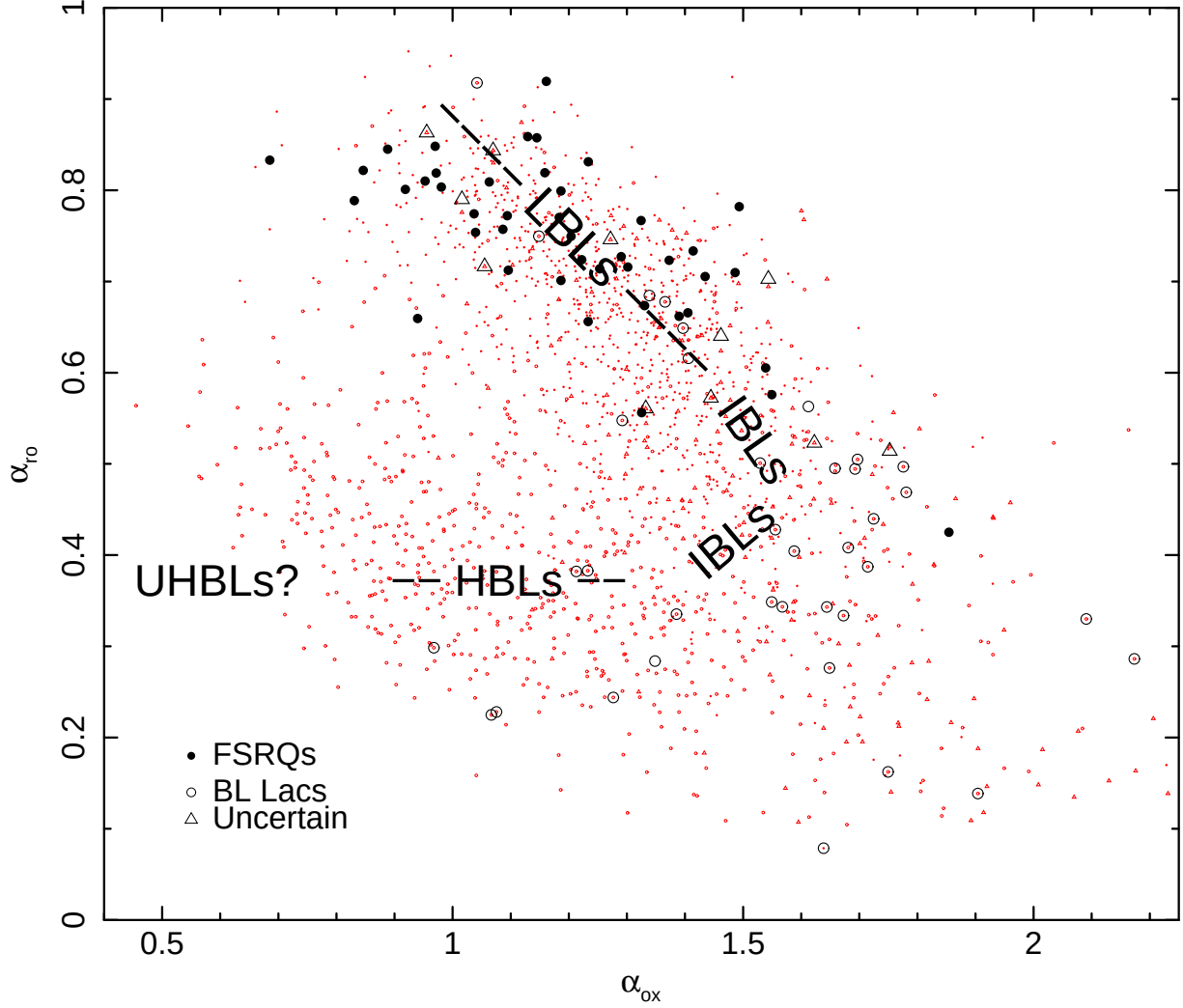
Fig. 27.— The \alpha_{\text{ox}} - \alpha_{\text{to}} plot of the LBAS blazars (large symbols) compared to the sample of blazars in the BZCAT catalog for which there is radio optical and X-ray information (small red symbols). All gamma-ray selected blazars are located in regions covered by previously known blazars. No new \gamma -ray type of blazars has been found, in particular there is no evidence for the hypothetical population of Ultra High energy peaked blazars (UHBLs), with synchrotron peak in the \gamma -ray band ( \text{Log}(\nu_{\text{peak}}^S) > 10^{20} Hz).
