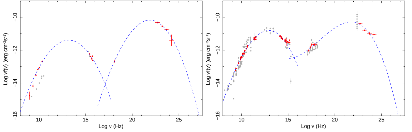
Fig. 5.— The SED of 0FGL J0349.8-2102 = PKS 0347-211 (left) and of 0FGL J0423.1-0112 = PKS0420-01 (right)
