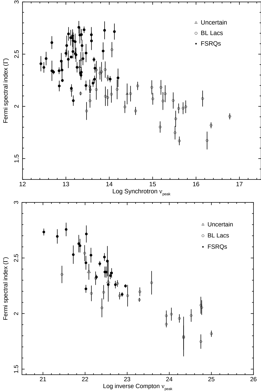
Fig. 29.— The \gamma -ray power law photon spectral index ( \Gamma ) is plotted against the log of synchrotron peak energy (top panel) and the Log of inverse Compton peak energy (bottom panel). A clear correlation is present in both cases. Note that BL Lacs behave differently than FSRQs spanning a wider range of both \nu_{\text{peak}}^S and spectral slopes.
