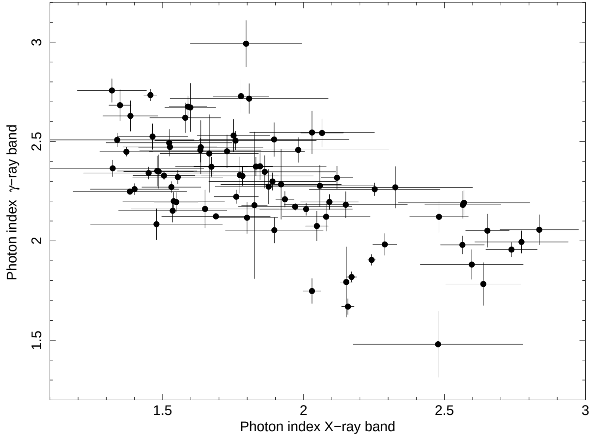
Fig. 35.— The power law spectral slope in the \gamma -ray band is plotted against the spectral slope in the X-ray band. A clear correlation is present.
