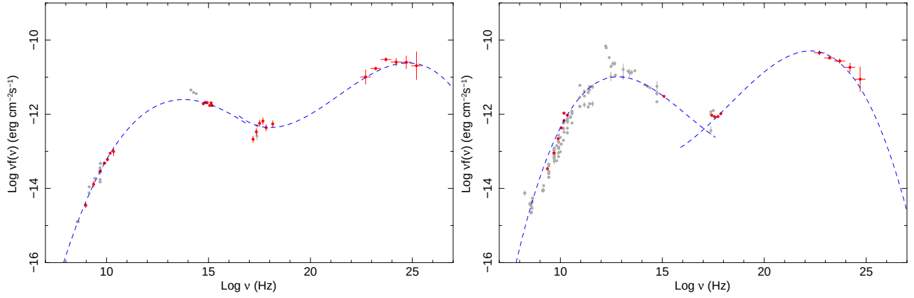
Fig. 20.— The SED of 0FGL J1719.3+1746 = PKS 1717+177 (left) and of 0FGL J1751.5+0935 = OT081
