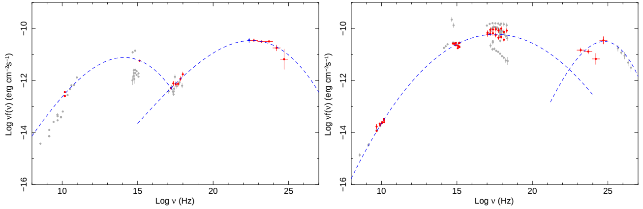
Fig. 21.— The SED of 0FGL J1849.4+6706 = 4C66.20 (left) and of 0FGL J2000.2+6506 = 1ES1959+650 (right)
