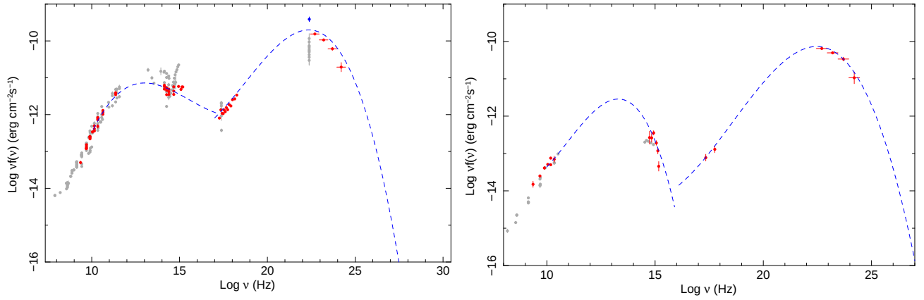
Fig. 18.— The SED of 0FGL J1512.7-0905 = PKS 1510-089 (left) and of 0FGL J1522.2+3143 = B2 1520+31 (right)
