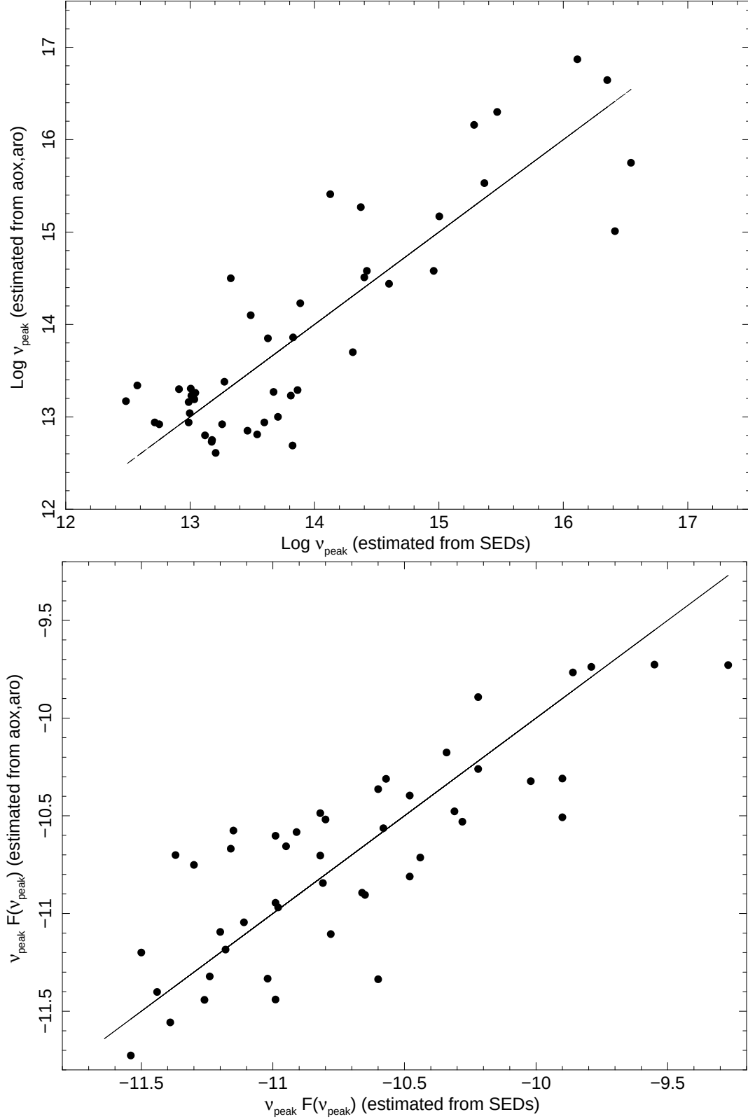
Fig. 28.— The synchrotron peak frequency ( \nu_{\text{peak}}^S , top panel) and its corresponding peak flux, \nu_{\text{peak}}^S F(\nu_{\text{peak}}^S) , bottom panel) value estimated from the SEDs of Figs. 1 through 24 is plotted against the value estimated using the method based on \alpha_{\text{ox}} and \alpha_{\text{ro}} values (see text for details). Despite the fact that \alpha_{\text{ox}} and \alpha_{\text{ro}} are based on non-simultaneous literature data, the scatter around the solid lines, representing perfect match, is \approx 0.6 and \approx 0.4 in log space for \nu_{\text{peak}}^S and \nu_{\text{peak}}^S F(\nu_{\text{peak}}^S)
