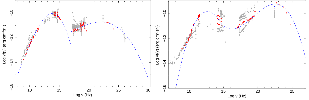
Fig. 23.— The SED of 0FGL J2202.4+4217 = BL Lacertae (left) and of 0FGL J2254.0+1609 = 3C454.3
