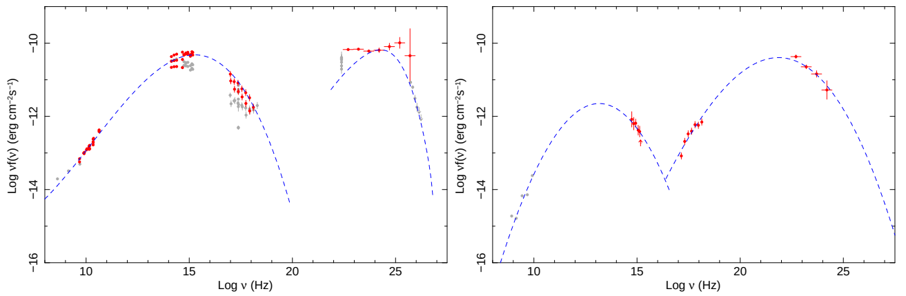
Fig. 3.— The SED of 0FGL J0222.6+4302 = 3C 66A (left) and of 0FGL J0229.5-3640 = PKS0227-369 (right)
