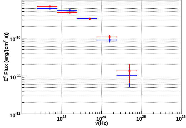
Fig. 37.— Comparison of the SEDs of the blazar 3C454.3 obtained with the maximum likelihood approach (red points) and with the unfolding technique (blue points).
