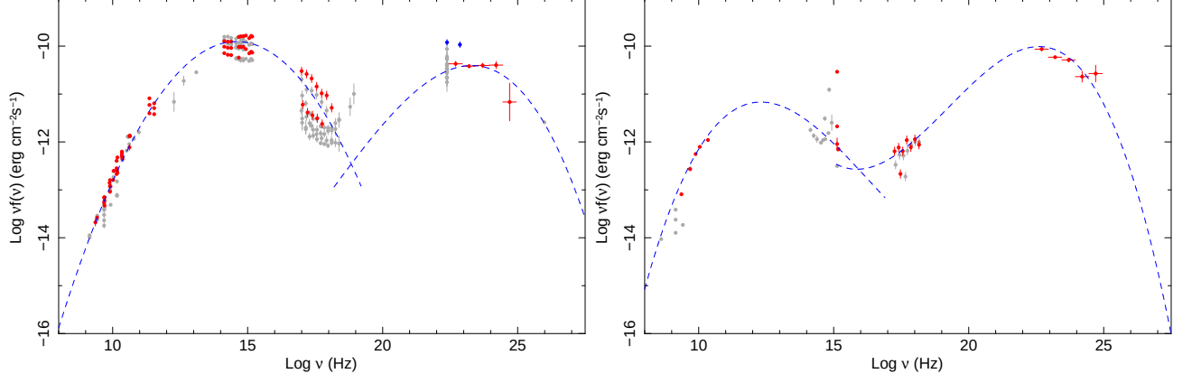
Fig. 10.— The SED of 0FGL J0722.0+7120 = S50716+714 (left) and of 0FGL J0730.4+1142 = PKS0727-11 (right)
