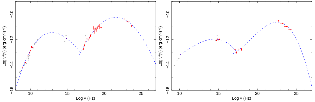
Fig. 24.— The SED of 0FGL J2327.3+0947 = PKS 2325+093 (left) and of 0FGL J2344.5-1559 = PMN J2345-1555 (right)
