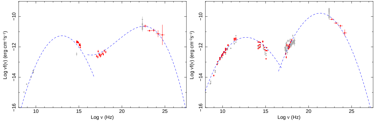
Fig. 8.— The SED of 0FGL J0516.2-6200 = MC4 0516-621 (left) and of 0FGL J0531.0+1331 = PKS 0528+134 (right)
