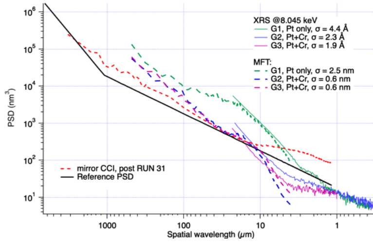
Figure 11: the measured PSDs on the coated samples, in comparison with the refence PSD for the BEaTriX mirror (black-solid line) and the state of the art of the uncoated mirror being polished (red-dashed line).
