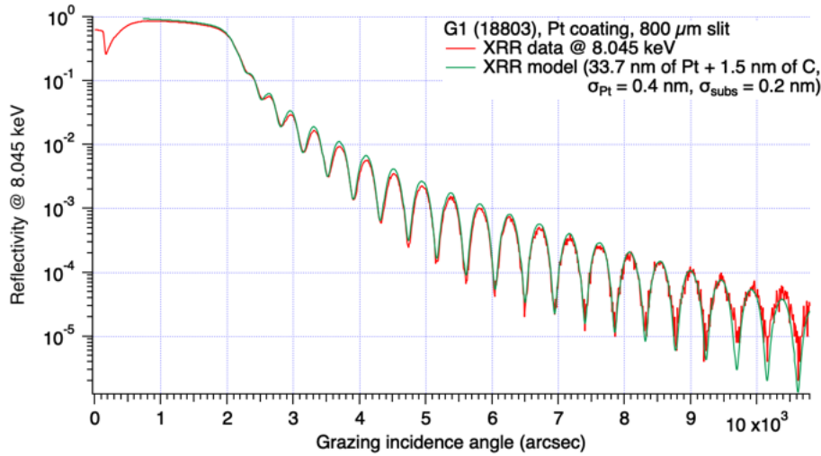
Figure 2: XRR measurement at 8.045 keV of the sample G1, with simple platinum coating. A thin layer of C contaminations had to be assumed, as suggested in the DTU report [AD1], in order to match the model to the experimental data at low incidence angles.
