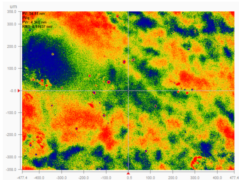
Figure 8: MFT 10x image sampled on G2 (platinum over chromium). The topography does not exhibit the defects seen on G1.
