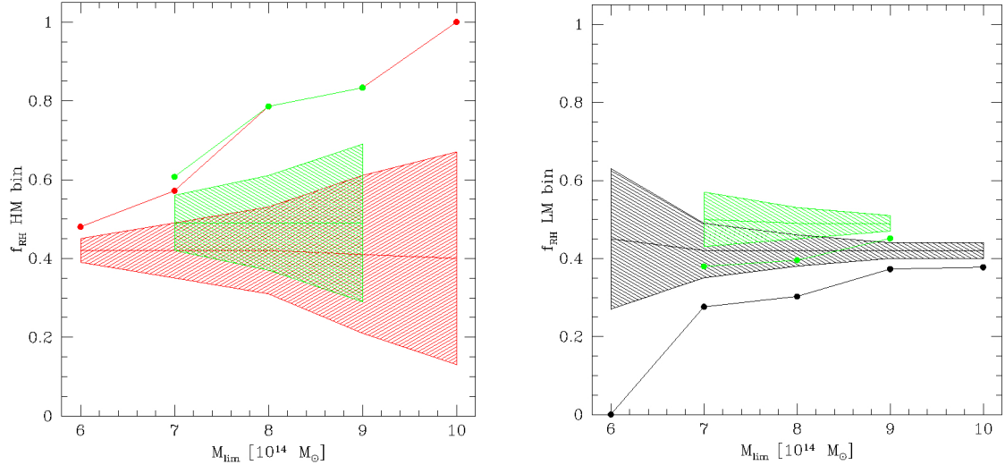
Fig. 5. Observed fraction of RHs f_{\text{RH}} (dots) compared to the value predicted by the Monte Carlo simulations (shadowed regions) in the HM bin (left panel) and in the LM bin (right panel) as a function of the limiting mass M_{\text{lim}} . In both panels the green dots and the green shadowed regions show the case in which the four clusters with suspect diffuse emission are considered as RH clusters.
