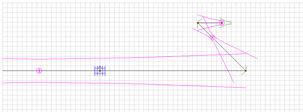
Figure 5: Layout of the Fore Optics ver.5. The red dot on the blue grid represent the location of the nominal Cassegrain focus for the band2 cartridge system. The magenta curves are the level at -12.00 dB of the beam propagated from the feed ( w_0 = 4 ) through the two reflectors.
