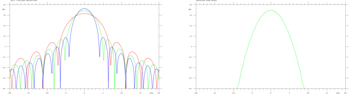
Figure 3: Horn models used for the calculation of ‘reference’ performances. The radiation pattern of a pure HE11 circular waveguide pattern is shown on the left at 67 GHz (red), 91.5 GHz (green) and at 116 GHz (blue). On the right the pure Gaussian radiation pattern is plotted at 91.5 GHz. Since it is defined by the taper angle the pattern is equal also at the other two frequencies.
