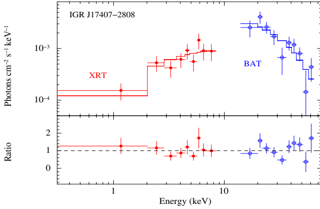
Fig. 8. Spectroscopy of the 2011 October 15 outburst of IGR J17407–2808. Top panel: simultaneous XRT/PC data (filled red circles) and BAT data (empty blue circles) fit with a PHABS*CUTOFFPL model. Bottom panel: the ratio between the data and the best-fit model.
