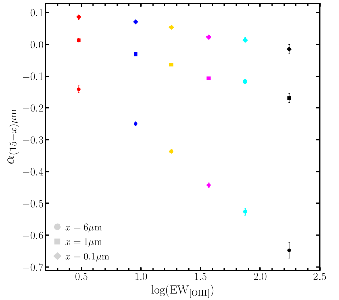
Figure 3. Energy slopes, as defined in equation (1), for the six stacked representative SED. The circles, squares, and diamonds indicate the slope (15–6) \mu\text{m} , (15–1) \mu\text{m} , and (15–0.1) \mu\text{m} , respectively.
