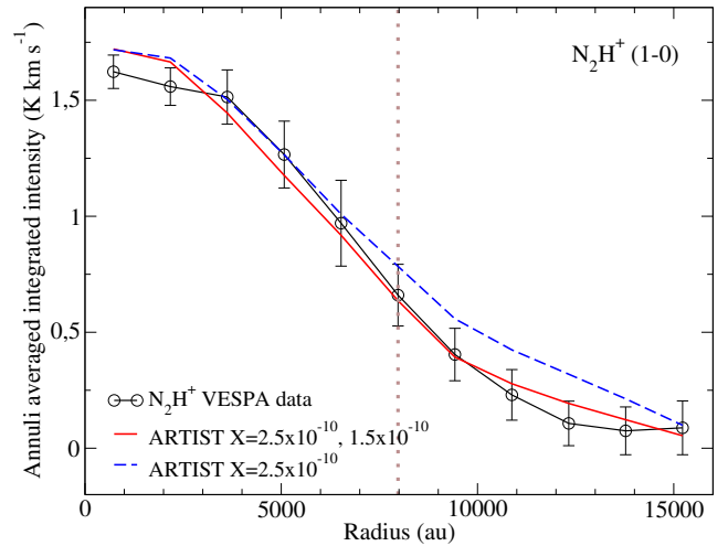
Fig. 8. \text{N}_2\text{H}^+ ARTIST abundance estimate. Annuli averaged integrated intensity vs. annuli radius. Black line: IRAM 30 m VESPA data. Blue dashed line: ARTIST radial integrated intensity profile for a constant abundance of 2.5 \times 10^{-10} . Red line: ARTIST radial integrated intensity profile with a step function abundance of 2.5 \times 10^{-10} and 1.5 \times 10^{-10} for smaller and larger radius than \sim 8000 \text{ au} (55 arcsec; indicated by the brown vertical dotted line), respectively.
