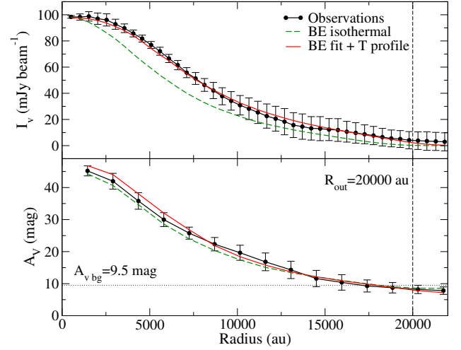
Fig. 6. Upper panel: intensity profile from the 1.2 mm dust continuum emission map (Frau et al. 2010, 2012b). Black line and dots: observed values with vertical bars depicting the \pm 1-\sigma range. Green (long-dashed) line: isothermal Bonnor-Ebert fit. Red (solid) line: fit Bonnor-Ebert profile adding the temperature profile shown in the upper panel of Fig. 7. The best fitting central density is \rho_c = 2 \times 10^5 \text{ cm}^{-3} . The fit core boundary radius, R_{\text{out}} = 20\,000 \text{ au} is marked by a vertical dashed line. Lower panel: A_v profile from the dust extinction map (Román-Zúñiga et al. 2009, 2010). Black, green (long-dashed) and red (solid) lines as in upper panel. The fit core boundary radius, R_{\text{out}} = 20\,000 \text{ au} , and A_v value of the surrounding medium, A_v^{\text{bg}} = 9.5 \text{ mag} , are labeled and marked by a vertical dashed line and horizontal dotted line, respectively.
