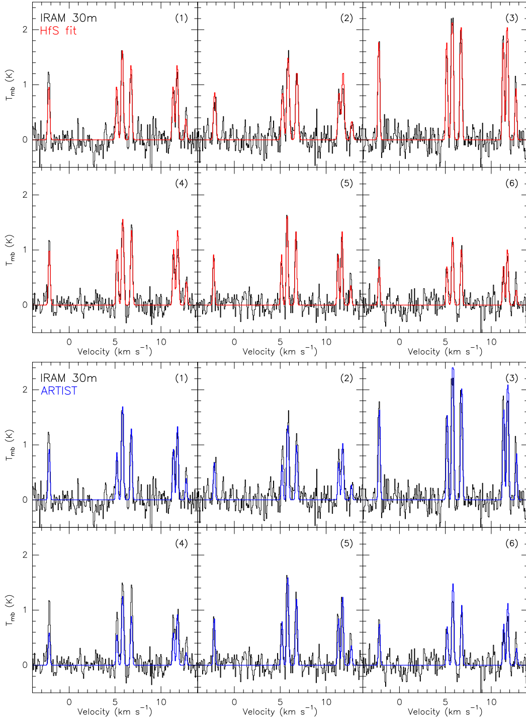
Fig. 2. Upper pannels: HfS fit of the hyperfine structure of \text{N}_2\text{H}^+ (1–0) IRAM 30 m spectral data at different positions of the core (labeled in Fig. 1c). Black and red lines are the observational data and the fit, respectively. Lower panels: ARTIST simulated \text{N}_2\text{H}^+ (1–0) spectral data (see Sect. 4.2). Black and blue lines are the observational and simulated data, respectively. We note that the simulated core from ARTIST is spherically symmetric. The discrepancies between the observational and the simulated spectra in panel (4) may be due to the slightly elongated shape of the core towards the west.
