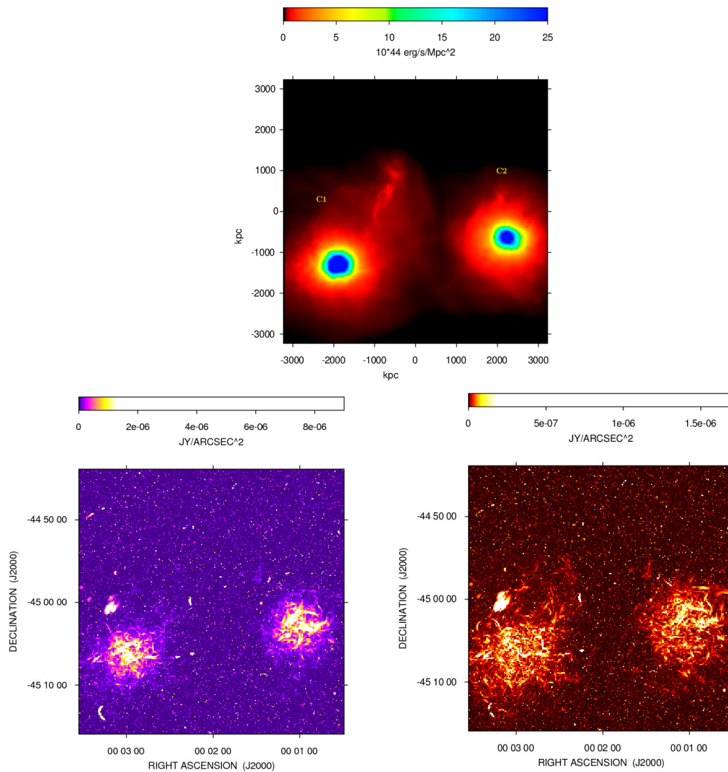
Figure 1. (a) X-ray surface brightness of a pair of galaxy clusters at redshift z = 0.205 , in a field of view of \sim 6.4 \text{ Mpc} with a spatial resolution of \sim 10.7 \text{ kpc} ; (b) total intensity surface brightness at 1.4 GHz of the cluster-embedded, foreground and background discrete radio sources plus the cluster radio halos; (c) polarized intensity surface brightness at 1.4 GHz of the cluster-embedded, foreground and background discrete radio sources plus the cluster radio halos. The beam Full-Width-at-Half-Maximum (FWHM) for images (b,c) is equal to 2.5'' , while the field of view is \sim 0.3 \text{ deg}^2 .
