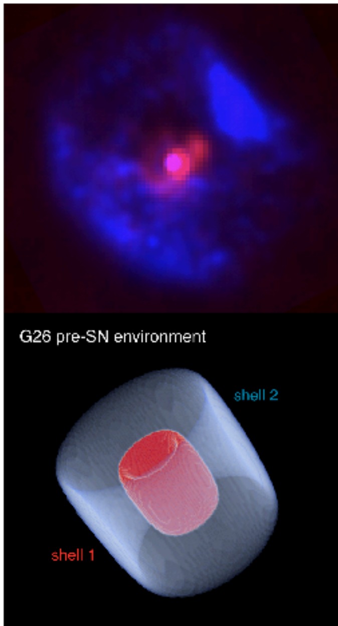
Fig. 2. Top: map of G26 which combines infrared at 24\ \mu\text{m} (blue) and radio (red) images (see Umama et al. 2012 ). Bottom: schematic view of the CSM around G26, representing the two dense shells (in red and light blue) observed in the radio and infrared bands. The LBV is located in the center of the two nested toroidal shells.
