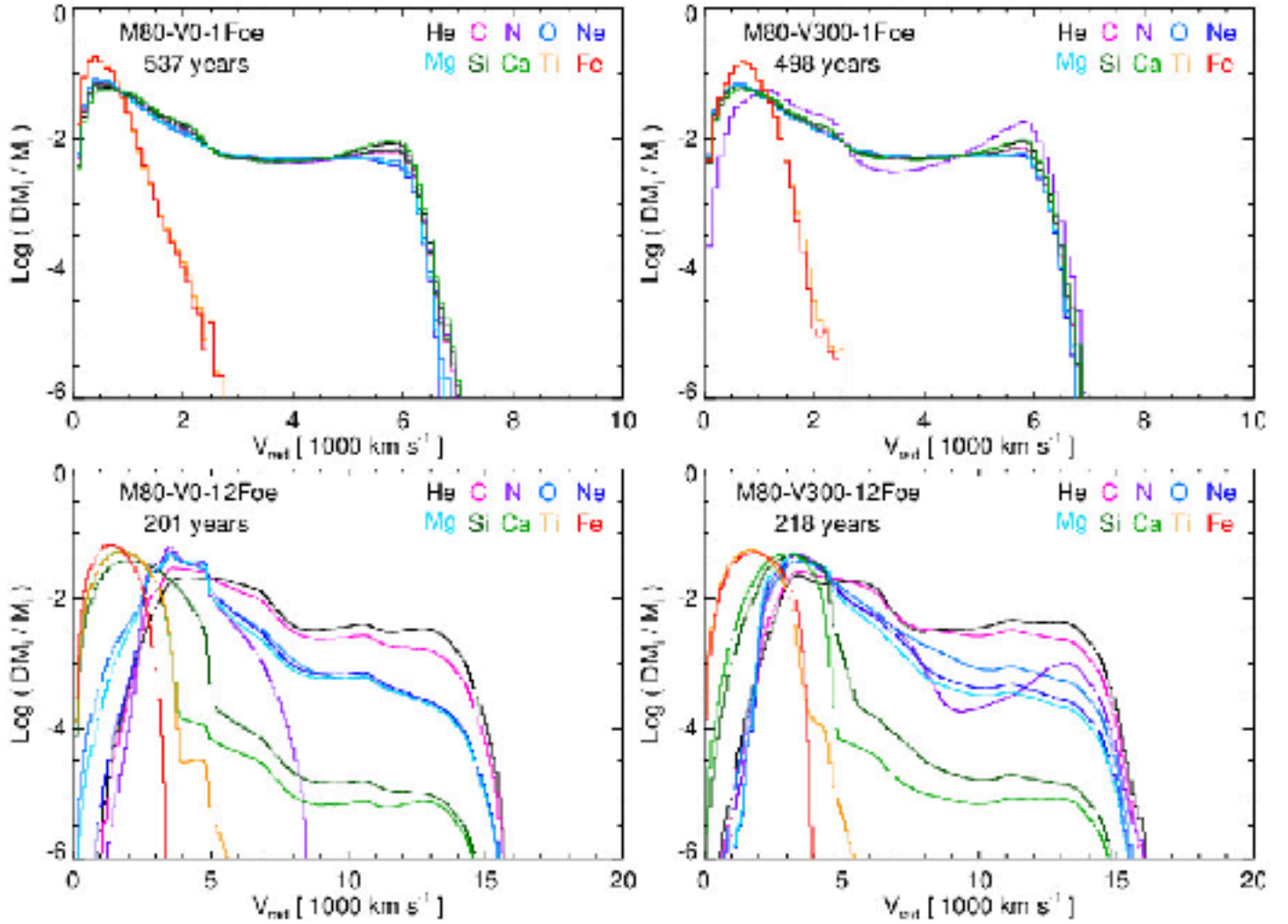
Fig. 11. Mass distributions of ^4\text{He} , ^{12}\text{C} , ^{14}\text{N} , ^{16}\text{O} , ^{20}\text{Ne} , ^{24}\text{Mg} , ^{28}\text{Si} , ^{40}\text{Ca} , ^{48}\text{Ti} , and ^{56}\text{Ni} versus radial velocity, V_{\text{rad}} , for models M80 at the time they reach their maximum degree of asymmetry. The figure shows models either with low ( upper panels ) or high ( lower panels ) explosion energy, and models either without ( on the left ) or with ( on the right ) initial rotation velocity of the star.
