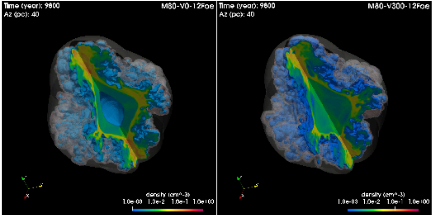
Fig. 7. Density distributions for the ejecta of the models M80-V0-12Foe (left panel) and M80-V300-12Foe (right panel) after \sim 10\,000 yr of evolution. The isosurfaces and the orientation of the system are defined as in Fig. 3.
