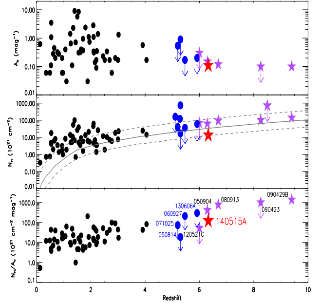
Fig. 9. A_V , N_{\text{H,X}} , and N_{\text{H,X}}/A_V ratio as a function of redshift. Black points are from Covino et al. (2013) for events with z \lesssim 4 , while the remaining events (blue circles, purple stars) are listed in Table 5. GRB 140515A is marked with a red star. The solid and/or dashed gray lines in the middle panel represent the effect of the intervening material along the line of sight (see Campana et al. 2015; Salvaterra 2015).
