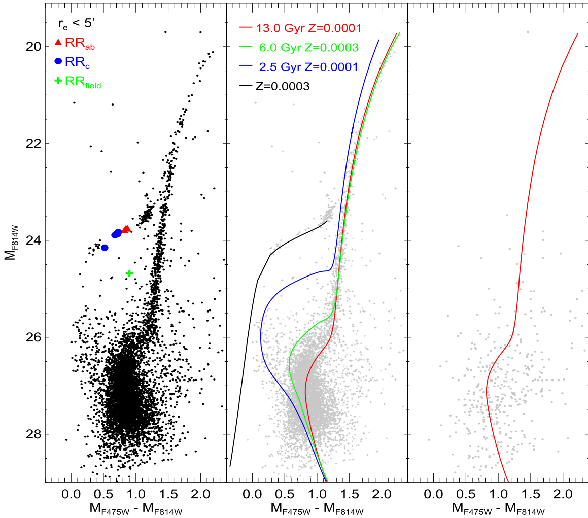
Figure 3. Left: CMD of And XVI, spanning from the tip of the RGB to well below the MSTO. Colored symbols show the RRL stars, with the same color code as in Figure 2. Middle: same CMD with superimposed selected isochrones from the BaSTI database, for labeled age and metallicity. The two selected isochrones bracket completely the TO region and the color spread of the RGB, suggesting a significant spread both in age and in metallicity. The black line shows the zero-age HB for Z = 0.0003 , which nicely reproduces the lower envelope of the HB stars. Right: CMD of the outermost region in the field of view, for r_e > 5' , where the majority of the detected sources are polluting unresolved background galaxies.
