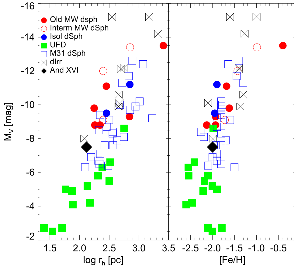
Figure 13. M_V magnitude vs. the logarithm of the half-light radius (left) and the metallicity (right) for LG dwarf galaxies of different morphological type. The data are from McConnachie (2012), but with updated values for And XVI. Different symbols indicate galaxies of different morphological types: red circle: MW dSphs (filled: purely old systems; open: systems with strong intermediate populations); blue circles: isolated dSphs (Cetus and Tucana); green squares: MW faint dwarf satellites; open squares: M31 dSph satellites; butterflies: dIrr systems (including transition types such as LGS3 and Phoenix).
