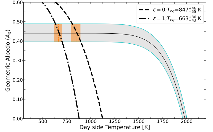
Fig. 3. Geometric albedo ( A_g ) estimated as a function of the day-side temperature for the measured occultation depth ( \delta_{\text{ecl}} = 6.95^{+0.66}_{-0.64} ppm). The cyan lines represent the 1\sigma uncertainty curves. The dash-dotted and dashed lines represent the variation of A_g with varying T_d for the 2 heat re-circulation cases ( \epsilon ) considered, computed at d = d_{\text{sec}} = 14.83 \pm 0.30 R_\star (that is, during the occultation). The 2 orange shaded regions correspond to the intersection of the curves, identifying the average HAT-P-11 b day-side temperatures for the 2 extreme scenarios of \epsilon , computed at d = d_{\text{sec}} . These 2 values of the equilibrium temperature with the associated uncertainties are reported in the legend.
