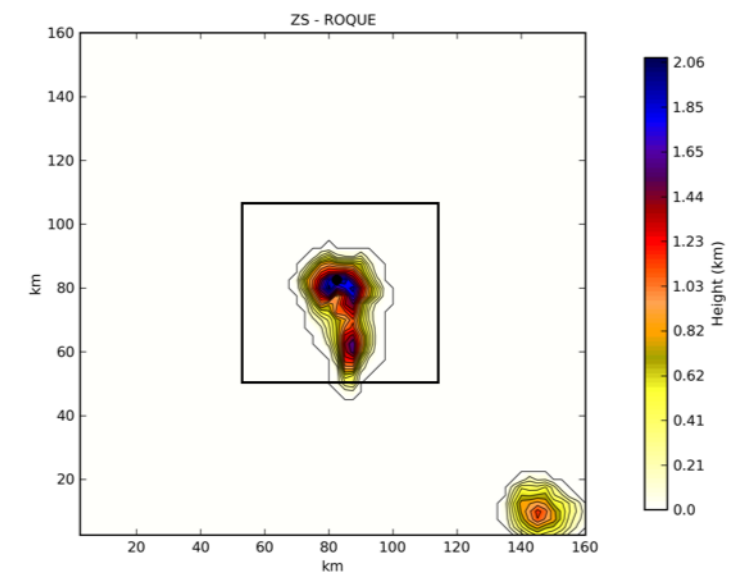
Fig. 4: La Palma Isle. The domain DOM2 extended on 160 km x 160 km i.e. 64 x 64 grid points with a resolution of 2.5 km. The black square indicates the most internal domain (DOM3).
