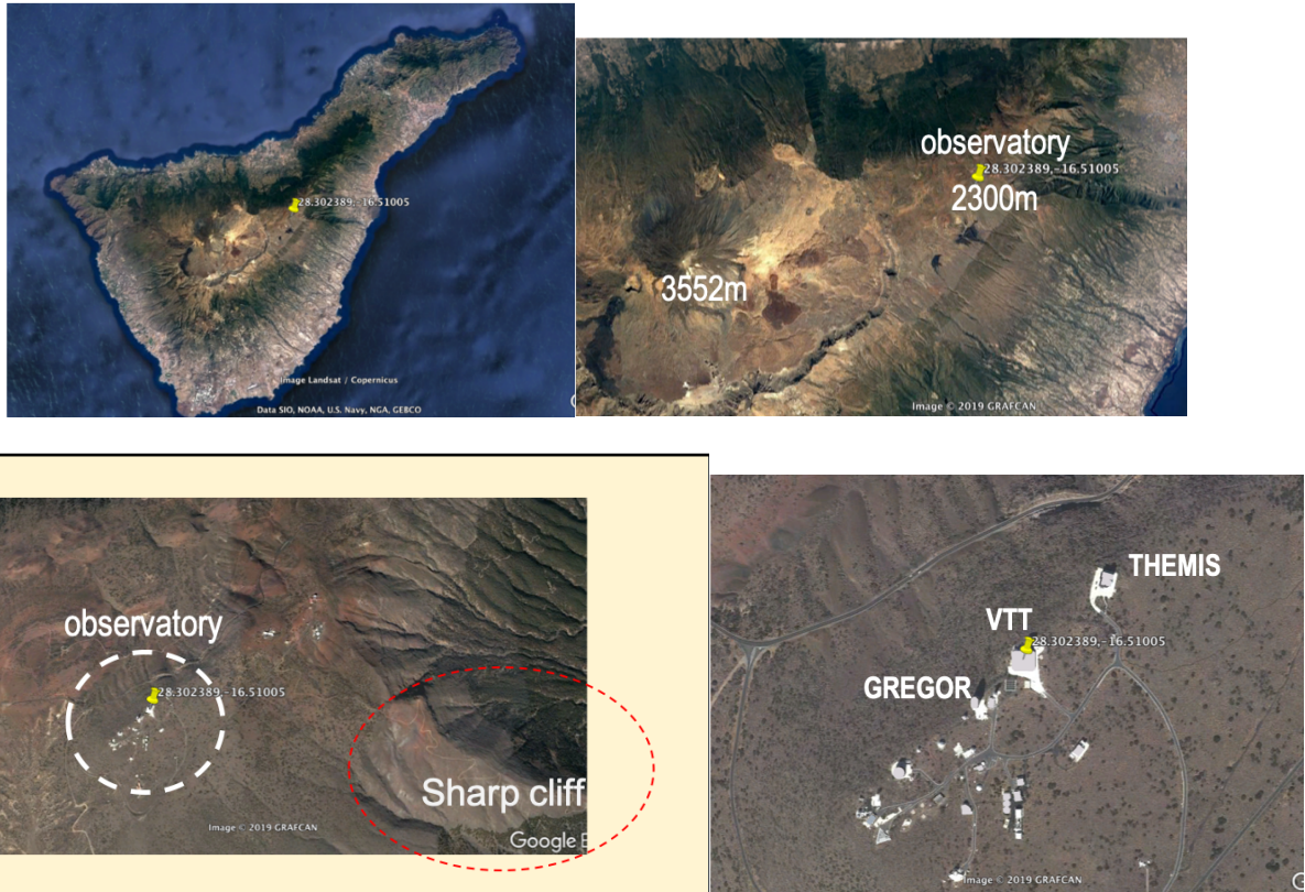
Fig. 10: Top-left: satellite view of the Tenerife Isle. Top-right: zoom of the region around the Teide Observatory in which it is visible a mountain on the West-side that is ~ 1 km higher than the TO summit. Bottom-left: a sharp cliff at the East with respect to the Teide Observatory. Bottom-right: position of the Vacuum Tower Telescope (VTT).
