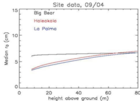
Fig. 23: Extracted from [RF9]. Median r_0 at different heights above the ground for La Palma.
