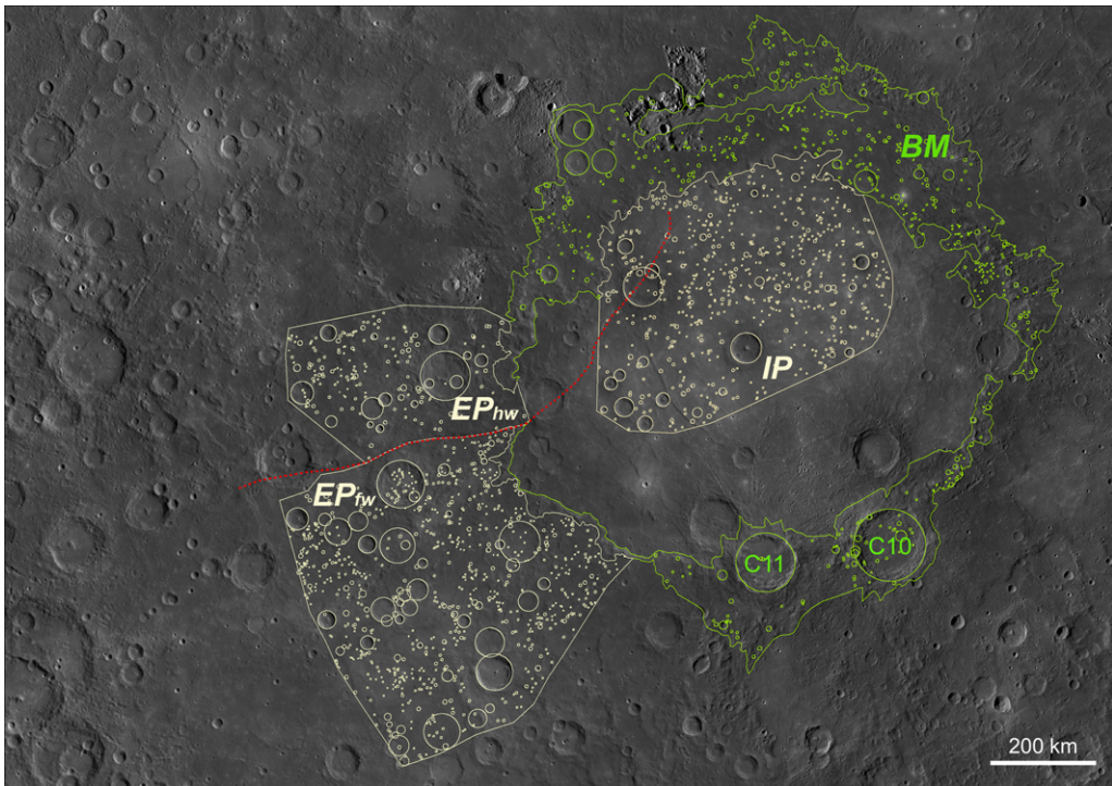
Fig. 3. Units in the Rembrandt basin region for which crater counts were performed, overlain on the MDS 750 nm mosaic (average spatial resolution: 250 m/pixel). The red dashed line marks the leading edge of the Enterprise Rupes system. The green line bounds the crater-counting area of basin-related materials (i.e. the Hummocky Material and Proximal Ejecta units) labelled as BM , and green circles indicate craters counted within this area. White lines bound the crater-counting areas of units affected by resurfacing: the IPa sub-unit counting area within the Rembrandt basin is labelled as IP ; counting areas located exterior to the basin are labelled EP fw at the footwall of Enterprise Rupes and EP hw at the hanging wall of the scarp; white circles indicate craters counted within this unit.
