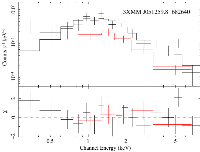
Fig. 3. EPIC pn and MOS2 spectra of 3XMM J051259.8–682640 from observation 0690742601 together with the best-fit model consisting of an absorbed power law.
