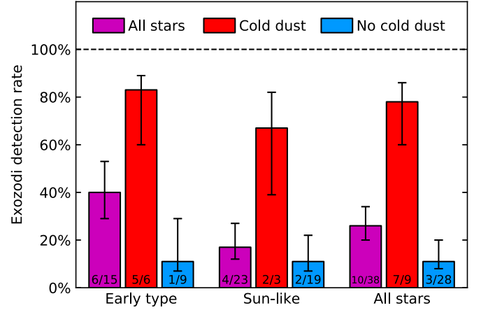
Figure 2. Histogram of HZ dust detection rates with respect to stellar spectral type and the presence of a detected, cold debris disk. The correlation between detection rate and spectral type is likely related to a sensitivity bias (Section 4.1). The correlation between detection rate and presence of cold dust is likely of astrophysical origin and found to be significant for early-type stars, while no conclusion can be drawn for Sun-like stars. The number of stars and detections in each subsample is indicated at the bottom of the corresponding bar.
