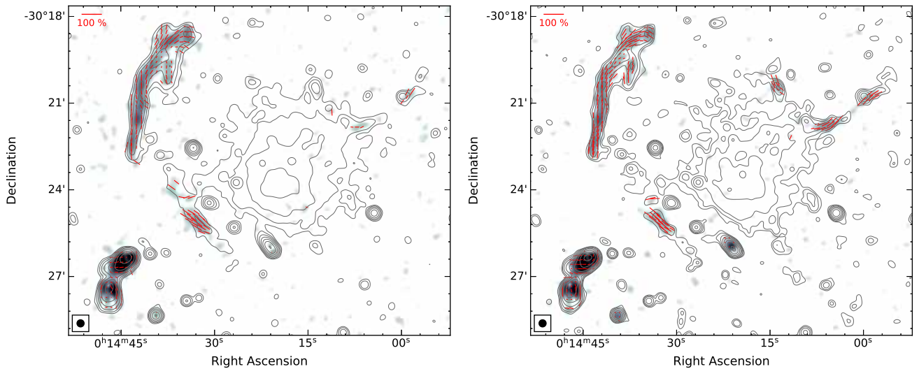
Fig. 18. VLA L-band (left) and S-band (right) polarization intensity maps at 15'' resolution. Red lines represent the magnetic field vectors. Their orientation represents the projected B-field corrected for Faraday rotation and the contribution from the Galactic foreground. For all four relics, the magnetic-field vectors are uniformly disturbed and parallel to the orientation of the radio emission. The vector lengths is proportional to the polarization percentage. No vectors were drawn for pixels below 3\sigma . Contour levels are drawn at [1, 2, 4, 8, \dots] \times 5\sigma_{\text{rms}} and are from the Stokes I images.
