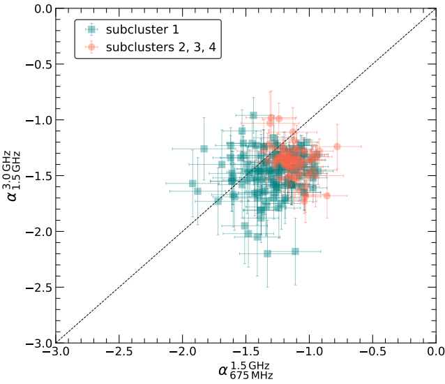
Fig. 12. Left: Radio color-color plot of the halo, showing a complex spectral curvature distribution. The orange data points are extracted from the southern part of the halo while turquoise one from the northern part. The curvature distribution is seems different in the northern and southern parts of the halo. Regions used for extracting the spectral index values are are shown in the right panel of Fig. 11. Right: Comparison between the radio (red) and the X-ray (blue) surface brightness profiles for the Abell 2744 halo. The X-radio and X-ray profiles are remarkably similar.
