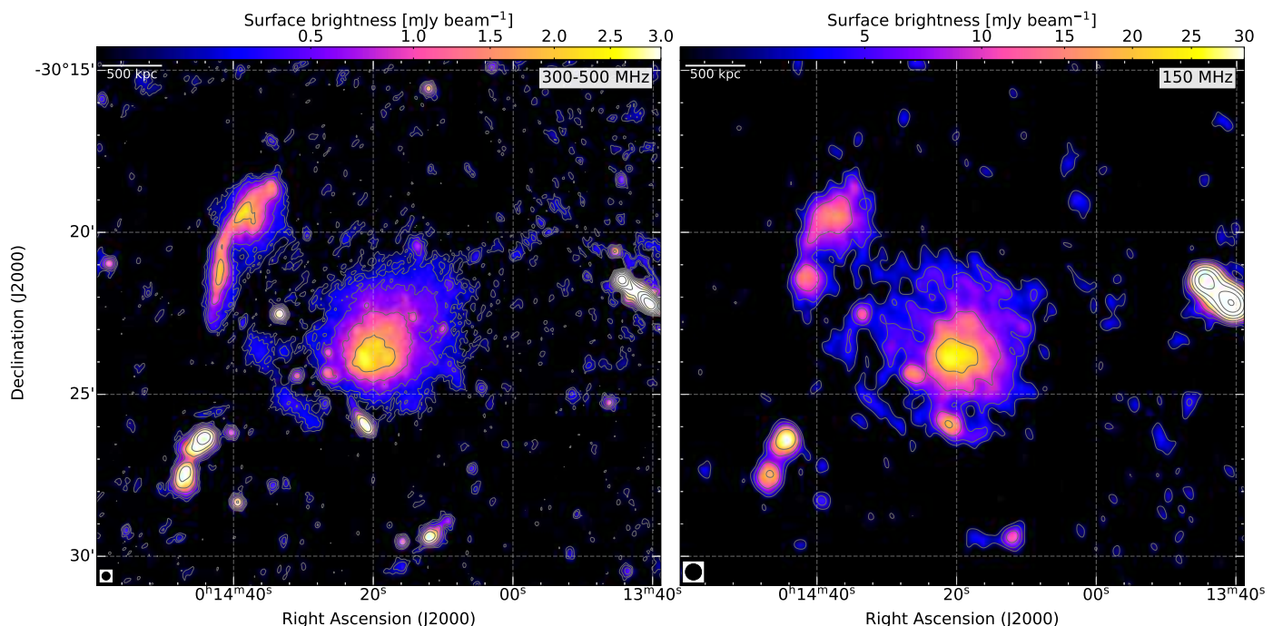
Fig. 4. uGMRT Band 3 (left) image at 15'' resolution and GMRT 150 MHz (right) narrow band image at 30'' resolution. The image properties are given in Table 2, IM16 (left-panel) and IM21 (right-panel). Contour levels are drawn at [1, 2, 4, 8, \dots] \times 3.5 \sigma_{\text{rms}} . In both images there is no region below -3.0 \sigma_{\text{rms}} . The halo and the main relic R1 are recovered well at both frequencies. Images are created with Briggs weighting with robust=0. The beam size is indicated in the bottom left corner of the each image.
