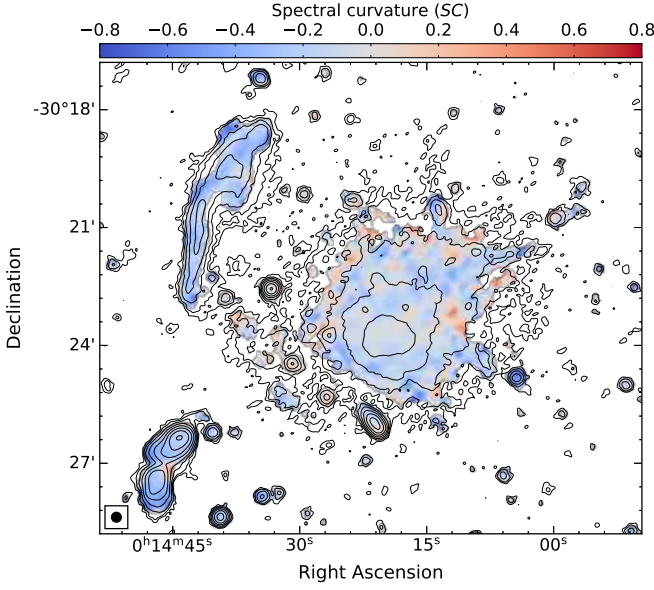
Fig. 11. Left: Three frequency spectral curvature map of the halo at 15'' resolution, created using 675 MHz, 1.5 GHz, and 3 GHz radio maps. The image properties are given in Table 2, IM3, IM7, and IM13. The halo shows a hint of spectral curvature. The SC is negative for a convex spectrum. Contour levels are drawn at [1, 2, 4, 8, \dots] \times 3.5 \sigma_{\text{rms}} , and are from the uGMRT Band 4 image. Right: Regions where the radio spectral index values were extracted between 675 MHz and 3 GHz. Each box has a width of 15'' corresponding to a physical size of about 67 kpc. The same regions are used to obtain \alpha - I_X correlation in the left panel of Fig. 15.
