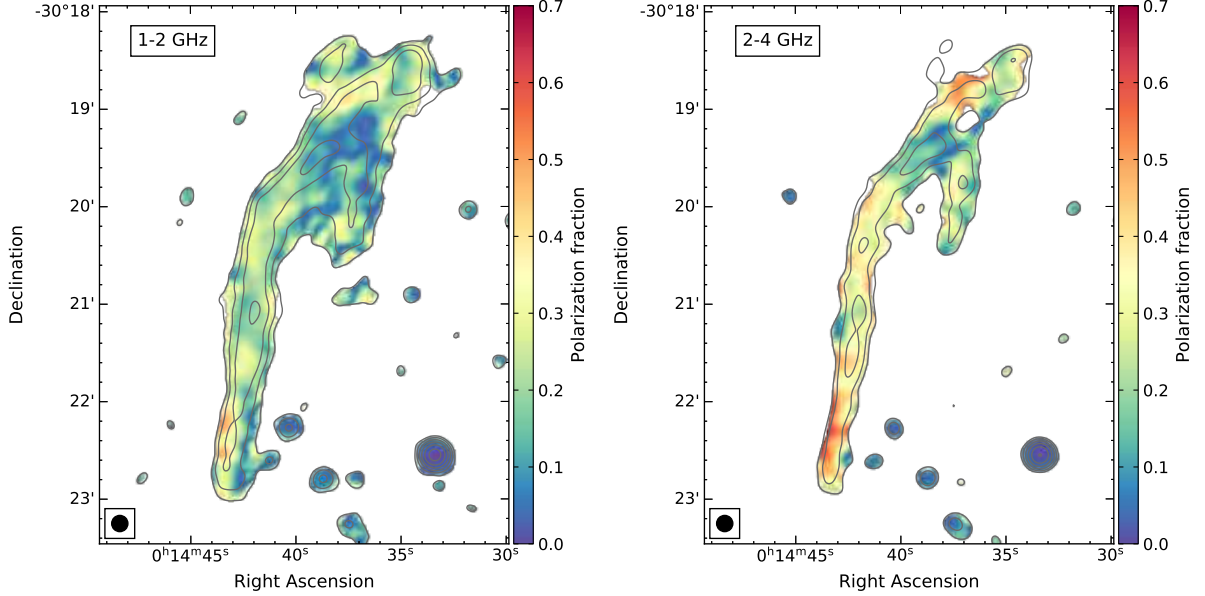
Fig. 17. Fractional polarization maps of the main relic at 10'' resolution. The degree of polarization across the relic decreases when going from S-band (right) to L-band (left). Some local fluctuations in polarization fraction are visible, particularly in the northern part of the relic. Contour levels are same as in Fig. 16.
