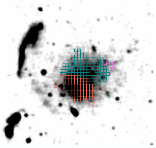
Fig. 11. Left: Three frequency spectral curvature map of the halo at 15'' resolution, created using 675 MHz, 1.5 GHz, and 3 GHz radio maps. The image properties are given in Table 2, IM3, IM7, and IM13. The halo shows a hint of spectral curvature. The SC is negative for a convex spectrum. Contour levels are drawn at [1, 2, 4, 8, \dots] \times 3.5 \sigma_{\text{rms}} , and are from the uGMRT Band 4 image. Right: Regions where the radio spectral index values were extracted between 675 MHz and 3 GHz. Each box has a width of 15'' corresponding to a physical size of about 67 kpc. The same regions are used to obtain \alpha - I_X correlation in the left panel of Fig. 15.
