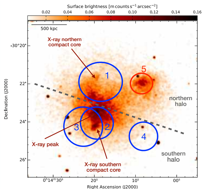
Fig. 1. Chandra 0.5 – 2.0 keV band image, smoothed with a Gaussian full width at half maximum (FWHM) of 3''. The cluster is rich in X-ray with several substructures near the center. Blue circles mark four subclusters detected in weak/strong lensing analysis ( Golovich et al. 2019 ). A fifth subcluster detected only in X-ray observations is shown with red circle. The dashed line represents the division between the northern (subclusters 1 and 5) and the southern (subclusters 2, 3, and 4) parts of the halo.
