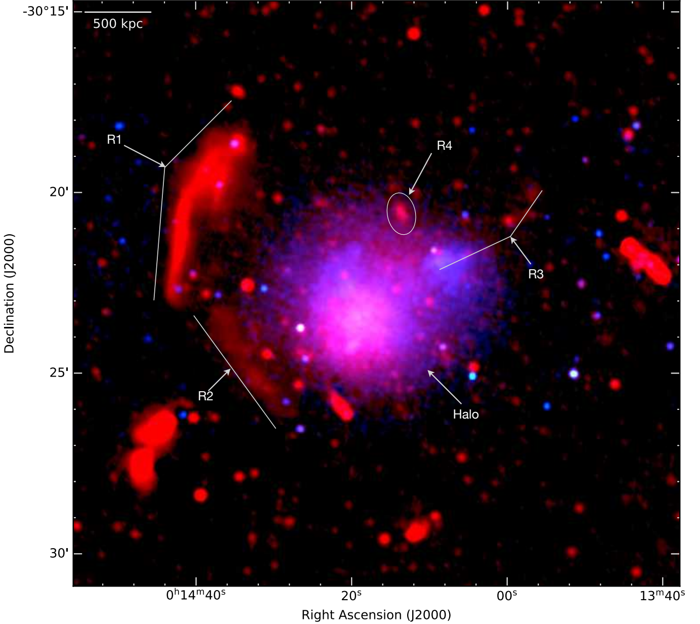
Fig. 2. Xray-uGMRT (550-850 MHz) overlay Abell 2744. The intensity in red shows the radio emission observed with uGMRT Band 4 at a central frequency of 675 MHz. The intensity in blue shows Chandra X-ray emission in the 0.5 – 2.0 keV band (Pearce et al. 2017), smoothed to 3". The image properties are given in Table 2, IM10. The presence of four relics and the halo suggests a complex, multiple mergers.
