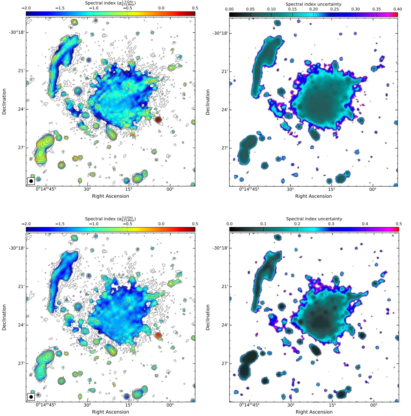
Fig. 9. Left: Spectral index maps of the halo between 675 MHz and 1.5 GHz (top) and 675 MHz and 3.0 GHz (bottom) at 15'' resolution. The image properties are given in Table 2, IM3, IM7, and IM13. Contour levels are drawn at [1, 2, 4, 8, \dots] \times 3.5 \sigma_{\text{rms}} , and are from the uGMRT Band 4 image. These maps show the presence of steeper spectral indices in outermost regions of the halo, in particular to the north. Right: Corresponding spectral index uncertainty.
