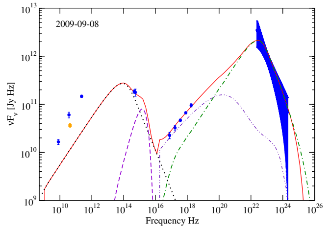
Figure 16. Spectral energy distributions (SEDs) of PKS 0528+134 corresponding to the first XMM-Newton observation. Blue points correspond to the observational data. The radio data correspond to the integrated radio flux from single-dish measurements. The orange radio point at 43 GHz is the flux of the VLBA core component. The continuous lines correspond to the best fit for each SED. The dotted line represents the synchrotron spectrum, the dot-dot-dashed line corresponds to the Synchrotron self Compton (SSC), the dot-dashed line is the external radiation Compton (ERC), and the short-dashed line is the disk thermal component.
