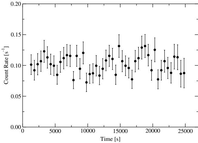
Figure 7. XMM-Newton MOS1 light curve of our ToO observation on 2009 September 10. Each point corresponds to a bin of 500 s. No evidence for intraday variability is found.
