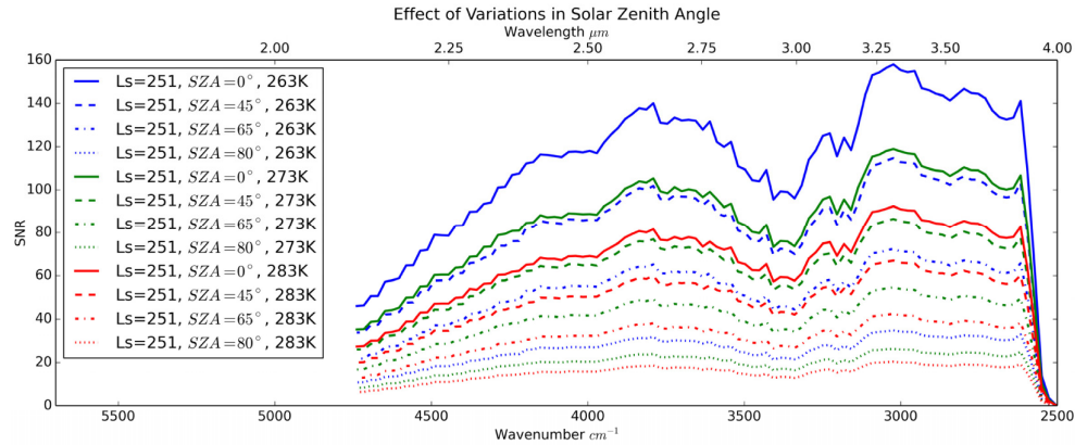
Fig. 11. Effects of Variations in Solar Zenith Angle: Expected SNR for LNO nadir observations for four solar zenith angles ( 0^\circ , 45^\circ , 65^\circ and 80^\circ ), one dust case ( OD = 0.2 ), intermediate surface albedo (0.242), one Sun-Mars distance (1.38AU @ L_s = 251^\circ ) and three instrument temperatures (263K, 273K and 283K).
