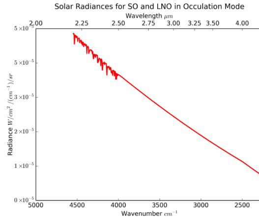
Fig. 3. Solar spectral radiance entering the SO and LNO solar occultation apertures. Note that radiance is invariant with Sun-Mars distance. Below 2.5 \mu m solar absorption lines are present in the spectrum.
