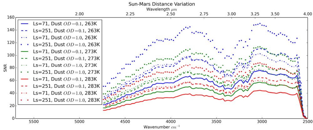
Fig. 9. Effects of Sun-Mars distance variations: Expected SNR for LNO nadir observations for one solar zenith angle ( 45^\circ ), two dust cases (OD = 0.1 and OD = 1), intermediate surface albedo (0.242), two Sun-Mars distances (1.38AU @ L_s = 251^\circ and 1.67AU @ L_s = 71^\circ ) and three instrument temperatures (263K, 273K and 283K).
