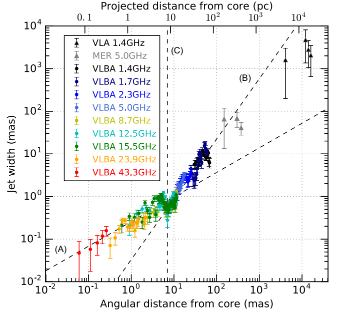
Figure 5. Extended plot of jet width profile of 1H 0323+342 including MERLIN and VLA measurements at large scales. The dashed lines (A), (B) and (C) are the same as in Figure 2.
