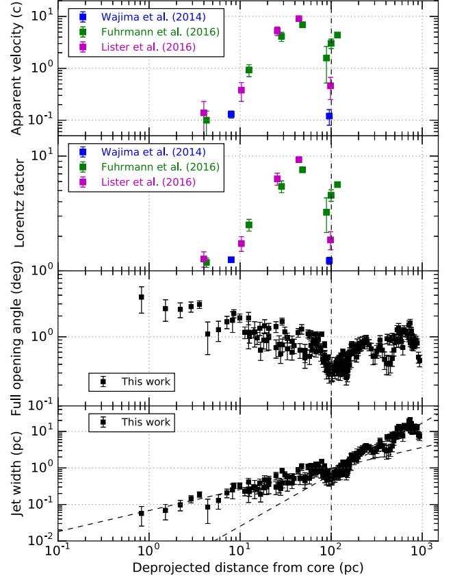
Figure 7. Collimation and acceleration of 1H 0323+342 jet as a function of deprojected distance from the core. A jet viewing angle of 5 deg is assumed. From the top panel to bottom: apparent motion reported in the literature; Lorentz factor calculated based on the apparent motion; intrinsic full opening angle calculated from the observed jet width profile; and jet width profile.
