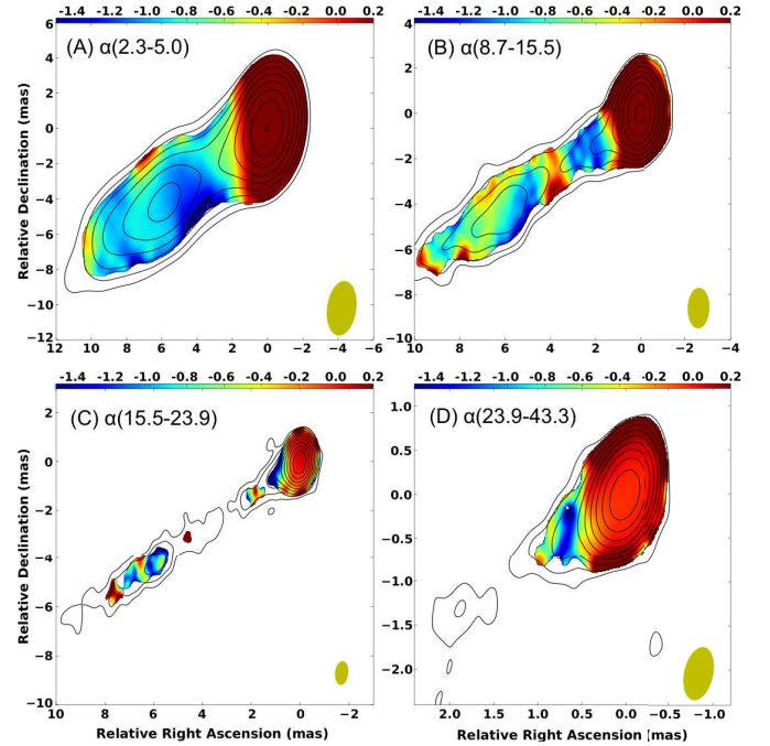
Figure 4. Spectral index (defined as S_\nu \propto \nu^{+\alpha} ) distribution of 1H0323+342 for various frequency pairs (color maps): (A) between 2.3 and 5.0 GHz; (B) between 8.7 and 15.5 GHz; (C) 15.5 and 23.9 GHz; (D) 23.9 and 43.3 GHz. Contours in each inset are a total intensity map at the lower frequency, starting from (1, 2, 4, 8, 16, 32, 64,...) times 0.2 mJy/beam. Yellow ellipse in each inset is the size of convolving beam.
